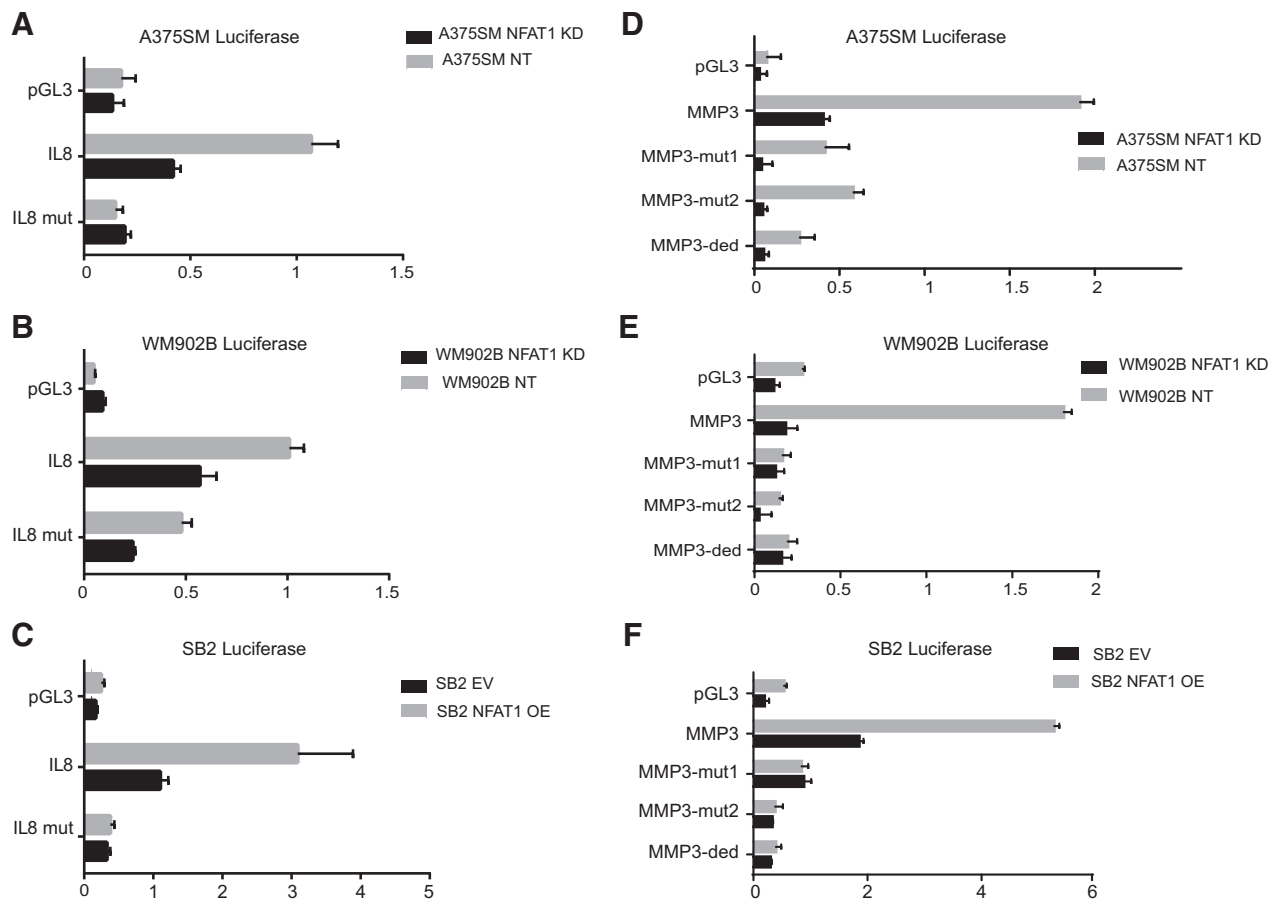
Figure 4. Effect of NAFT1 on IL8 and MM-3 promoter activities. A and B, silencing NFAT1 in both A375SM and WM902B cells significantly reduced the luciferase activity driven by the wild-type IL8 promoter by approximately 75% compared with NT shRNA. Mutating NFAT1-binding sites (each one separately or both) resulted in reduced promoter activity compared with the wild-type promoter ( P < 0.05 ). A, A375SM melanoma cells. B, WM902B melanoma cells after silencing NFAT1. C, SB2 melanoma cells after overexpressing NFAT1. D and E, silencing NFAT1 in both A375SM and WM902B cells significantly reduced the luciferase promoter activity of the wild-type MMP3 promoter by approximately 50% compared with NT shRNA ( P < 0.05 ). Mutating the NFAT1-binding site at location -32 from the TIS resulted in reduced promoter activity to approximately 50% of the wild-type promoter ( P < 0.05 ). F, NFAT1 overexpression in SB2 cells increased luciferase promoter activity.
