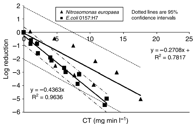
Figure 5 | Monochloramine inactivation of Nitrosomonas europaea ATCC 19718 and Escherichia coli O157:H7 in particle-free reactors (pH 8.0, 21°C). The slopes of the inactivation kinetics of the two conditions were statistically different within a 95% confidence level ( t -test).
