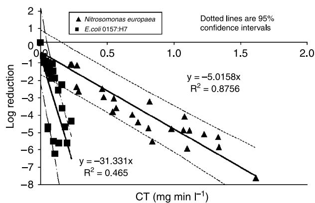
Figure 6 | Chlorine inactivation of Nitrosomonas europaea ATCC 19718 and Escherichia coli O157:H7 in particle-free reactors (pH 7.0, 21°C). The slopes of the inactivation kinetics of the two conditions were statistically different within a 95% confidence level ( t -test).
