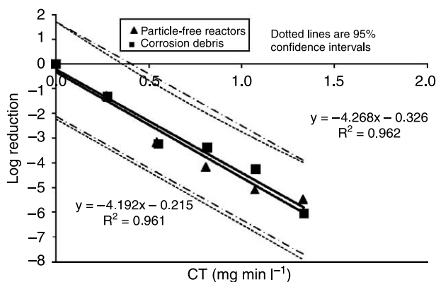
Figure 4 | Inactivation of Nitrosomonas europaea ATCC 19718 by chlorine (pH 7.0, 21°C) in particle-free reactors or in the presence of 50 mg l -1 of corrosion debris. The slopes of the inactivation kinetics of the two conditions were statistically the same within a 95% confidence level ( t -test).
