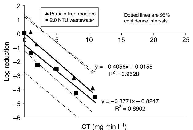
Figure 3 | Inactivation of Nitrosomonas europaea ATCC 19718 by monochloramine (pH 8.0, 21°C) in particle-free reactors or in the presence of 2.0 NTU wastewater. The slopes of the inactivation kinetics of the two conditions were statistically the same within a 95% confidence level ( t -test).
