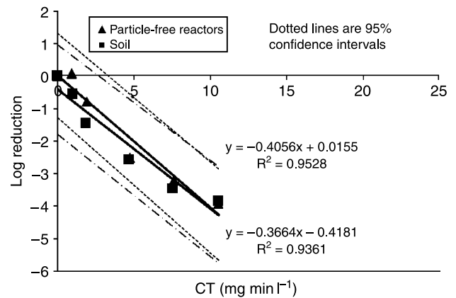
Figure 2 | Inactivation of Nitrosomonas europaea ATCC 19718 by monochloramine (pH 8.0, 21°C) in particle-free reactors or in the presence of 50 mg l -1 of soil. The slopes of the inactivation kinetics of the two conditions were statistically the same within a 95% confidence level ( t -test).
