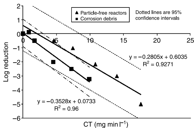
Figure 1 | Inactivation of Nitrosomonas europaea ATCC 19718 by monochloramine (pH 8.0, 21°C) in particle-free reactors or in the presence of 50 mg l -1 of corrosion debris. The slopes of the inactivation kinetics of the two conditions were statistically the same within a 95% confidence level ( t -test).
