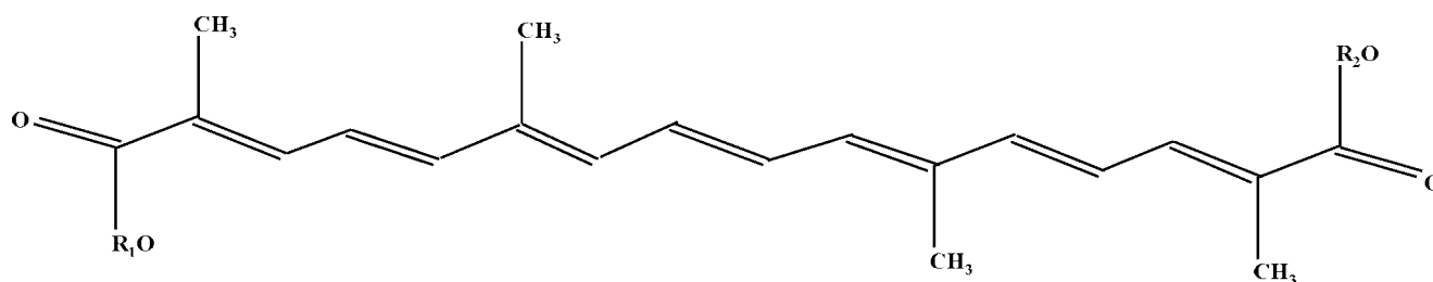
Figure 1. Known chemical structures of crocetin separated from Saffron by Tarantilis et al. (14).
