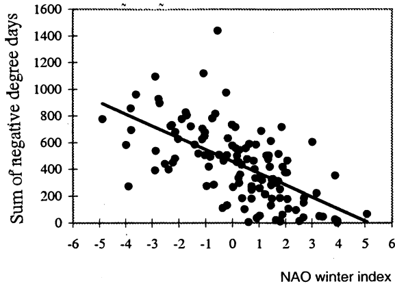
Fig. 2. Relation between time series of sum of negative degree-days in Pärnu and the NAO winter index.
