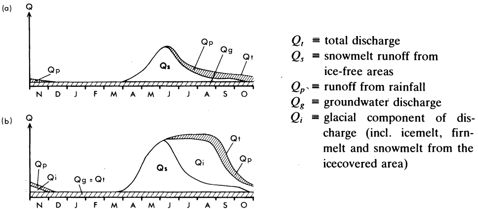
Fig. 1. (a) Schematic annual discharge hydrograph of a stream draining a nival catchment, with seasonal snow cover, but no perennial ice storage.
