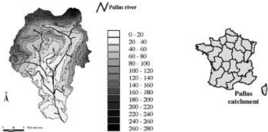
Figure 1 Pallas catchment location (Hérault, France)
