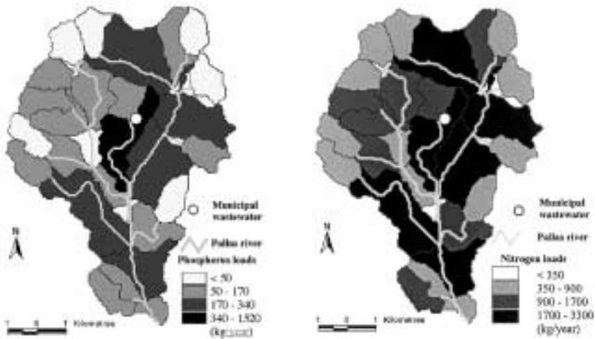
Figure 3 Subcatchment delineation with annual phosphorus and nitrogen loads estimation (kg/year)
