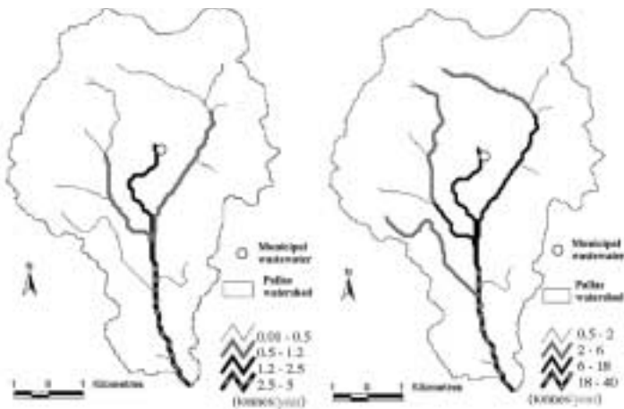
Figure 4 Hydrographic network with annual phosphorus and nitrogen quantity estimation (tonnes/year)
