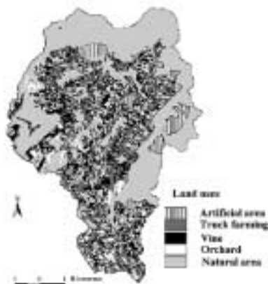
Figure 2 Land uses of Pallas watershed obtained from SPOT classification, an associated specific "nutrient generation rate" (Benneton, 1984)
