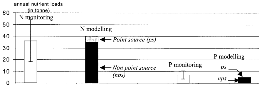
Figure 5 Comparison between annual nutrient load estimates by our modelling approach and by water quality monitoring
