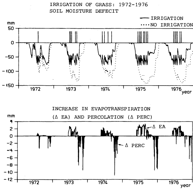
Fig. 13. Irrigation of grass 1972-76.
