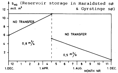
Fig. 7. Strategy for transfer of water from Tystrup sø to Gyrstinge sø and transmission intensities.
