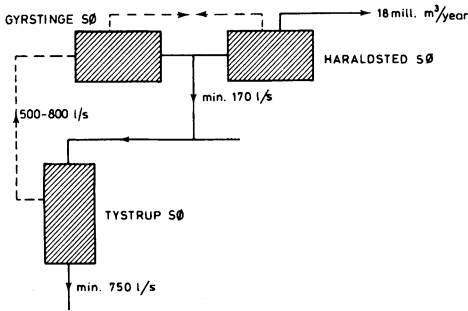
Fig. 7. Strategy for transfer of water from Tystrup sø to Gyrstinge sø and transmission intensities.
