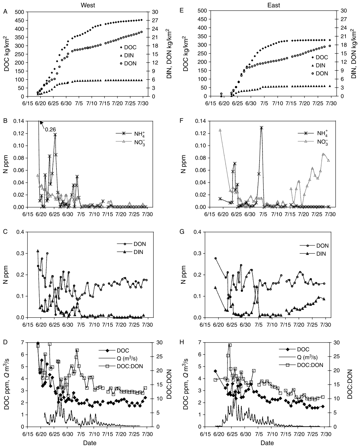
Figure 2 | Seasonal variations in dissolved solute fluxes (kg/km 2 ), concentrations (ppm) and discharge (m 3 /s) in the West and East rivers. Cumulative specific mass fluxes of DOC, DON and DIN are shown in panels (A) and (E). Concentrations of N from NO 3 - and NH 4 + are shown in panels (B) and (F). DIN and DON concentrations are plotted in (C) and (G). DOC concentrations are plotted with mean daily discharge and DOC:DON (secondary y axis) in panels (D) and (H).
