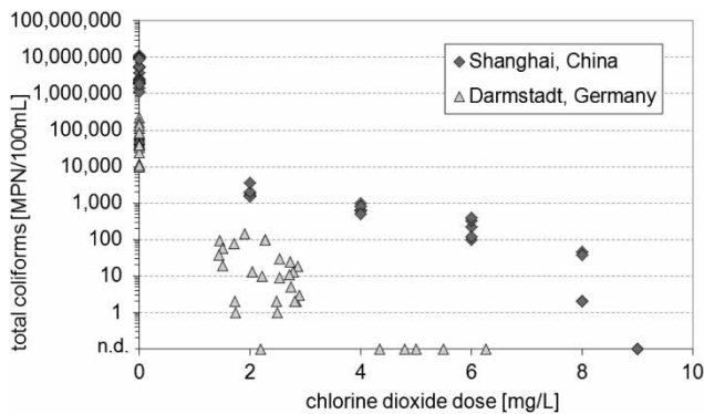
Figure 3 | Concentrations of total coliforms as a function of ClO 2 dose.
