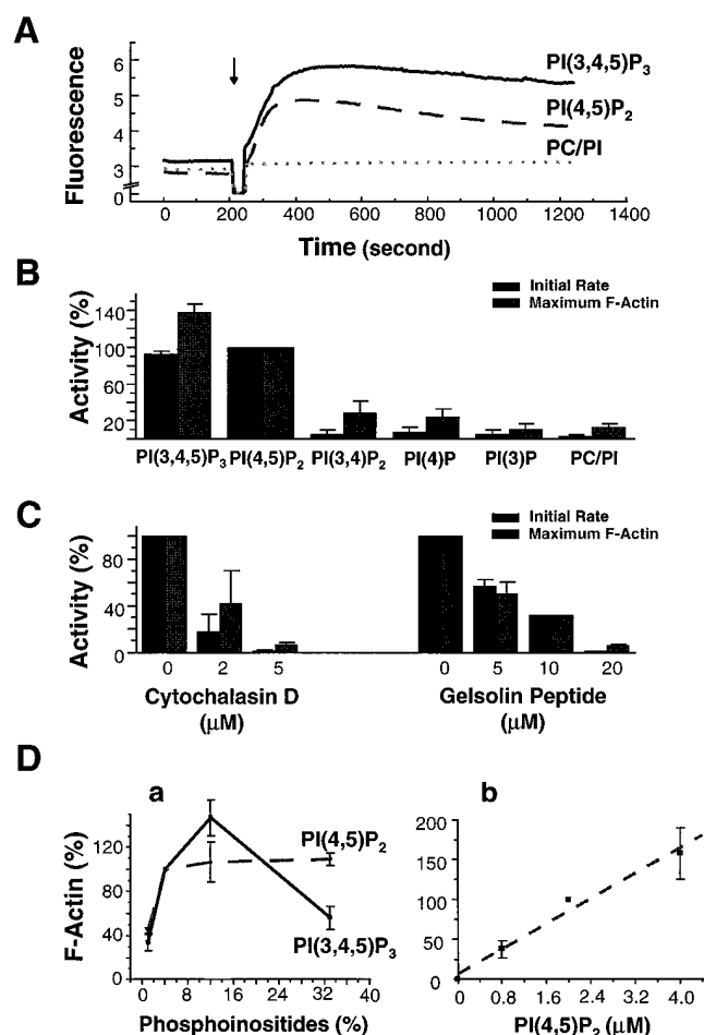
Figure 3. Characterization of phosphoinositide-induced actin assembly in high speed supernatants using pyrene actin. (A) Time course of change in pyrene fluorescence in high speed supernatants treated with PC/PI alone (dotted line), or PC/PI vesicles containing 4% PI(3,4,5)P 3 (solid line), or 4% PI(4,5)P 2 (dashed line). The lipid concentration was 50 \mu\text{M} . The arrow indicates the time when the lipid was added. (B) Comparison of the inductive activity among different phosphoinositides in PC/PI vesicles (4% phosphoinositides in 50 \mu\text{M} total lipids) as measured by the initial rate of actin assembly and the maximum F-actin at the peak. All activities are normalized to that of PI(4,5)P 2 . (C) Inhibition of PI(4,5)P 2 -induced actin assembly in high speed supernatants by cytochalasin D or a peptide (QRLFQVKGR) derived from gelsolin. Each reaction included 50- \mu\text{M} lipid vesicles containing 4% PI(4,5)P 2 . Inhibition of PI(3,4,5)P 3 -induced activity is similar and is not shown here. (D) Dose response of actin assembly to phosphoinositides. (a) F-actin induced by 50- \mu\text{M} PC/PI vesicles containing different percentages of PI(3,4,5)P 3 (solid line) or PI(4,5)P 2 (dashed line). (b) F-actin induced by vesicles containing 4% PI(4,5)P 2 in high speed supernatants at various total lipid concentrations (expressed as total PI(4,5)P 2 ). The data fit into a linear curve (dashed line). The initial rate has very similar dose-response profiles (not shown). All activities are normalized to that of phosphoinositides at 4% in 50 \mu\text{M} total lipids. All data in B–D are expressed as mean \pm SEM calculated from at least two sets of normalized data.
