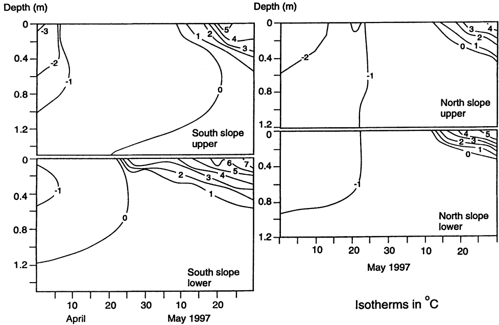
Fig. 4. Temperature changes in the near surface zones at four plots. For each plot, the disappearance of its snow cover corresponded with the rise of the surface temperature above 0°C.
