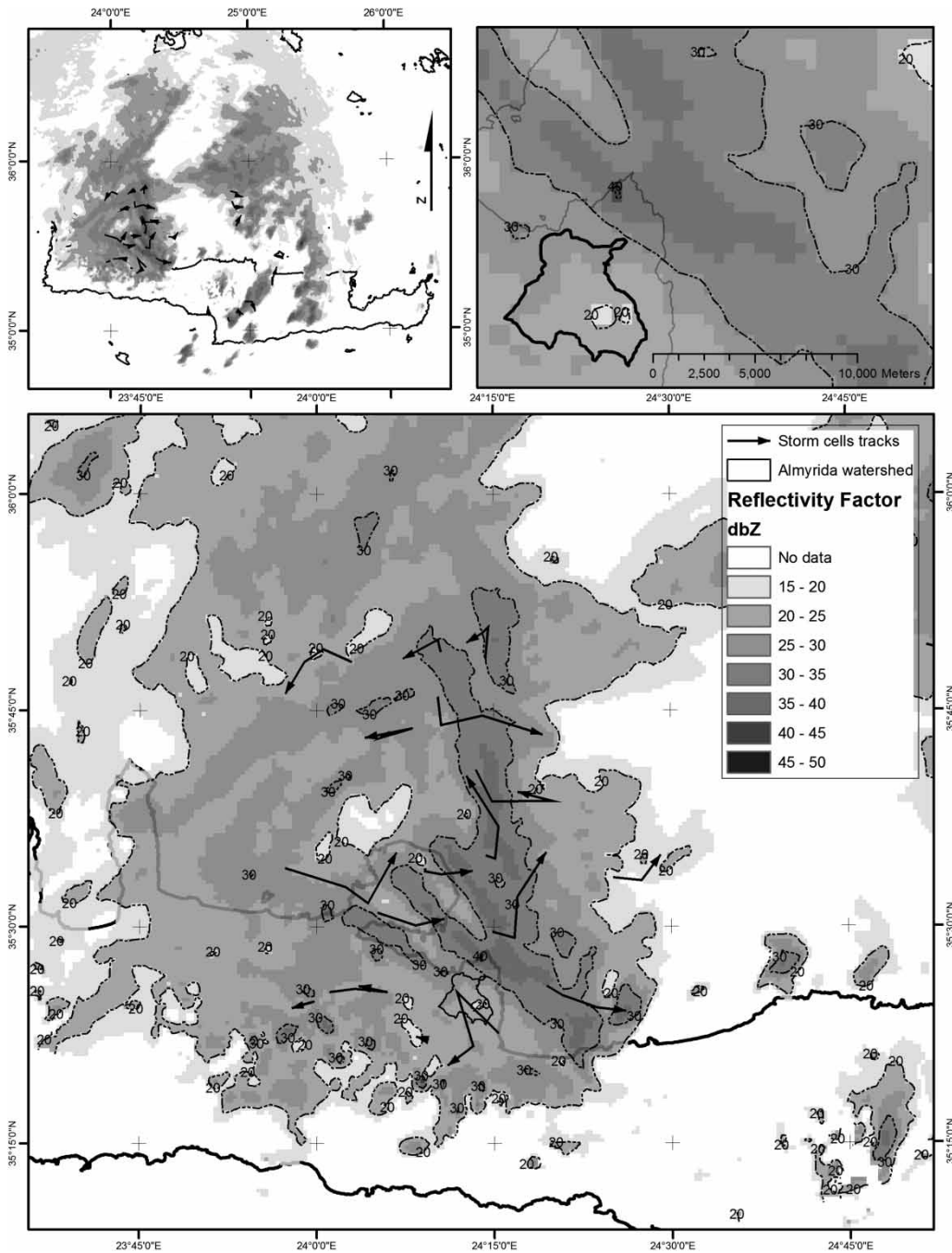
Figure 5 | Reflectivity of the storm that hit the north coast of Crete on October 17, 2006 as it was recorded on 15:13 UTC. Arrows show the direction of individual storm cells from 15:13 to 15:58 UTC.
