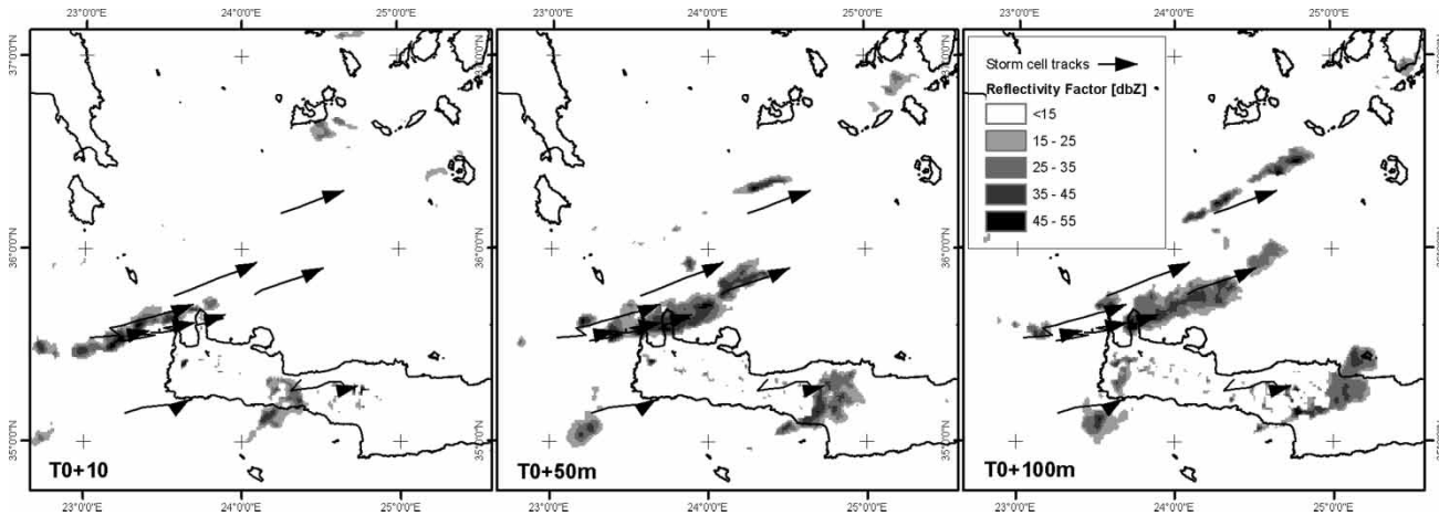
Figure 3 | Storm cell center detection and tracking during a 100 m interval consisting of 10 radar scans (only three shown).
