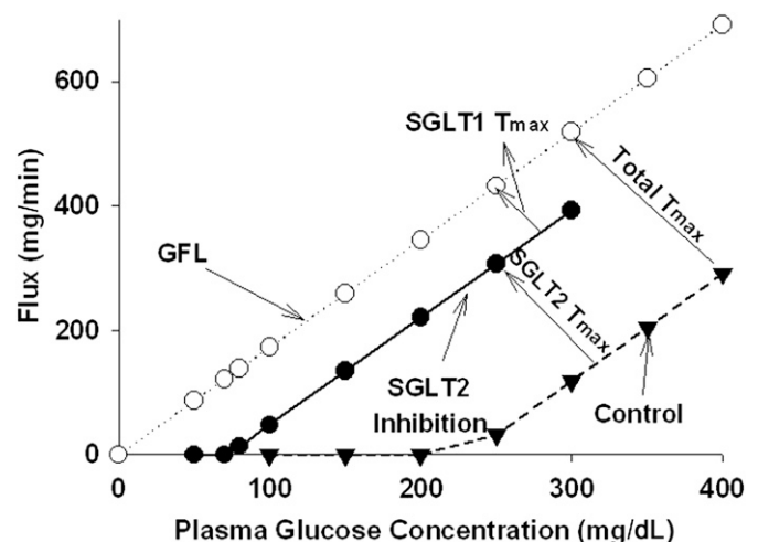
FIG. 2. Relationship between glucose filtration load (GFL) and UGE and the plasma glucose concentration under physiologic conditions and during maximal inhibition of SGLT2.
