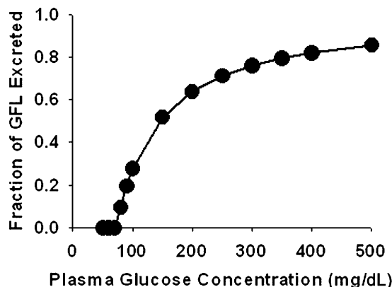
FIG. 4. Predicted relationship between the fraction of filtered glucose excreted in the urine and the plasma glucose concentration during maximal inhibition of SGLT2. The maximal SGLT1 transport capacity was estimated at 120 g/day (see text for details). GFL, glucose filtration load.
