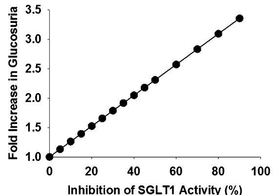
FIG. 5. Predicted fold increase in the level of glucosuria produced by SGLT2 inhibitors in relation to the percent inhibition of SGLT1 activity.
