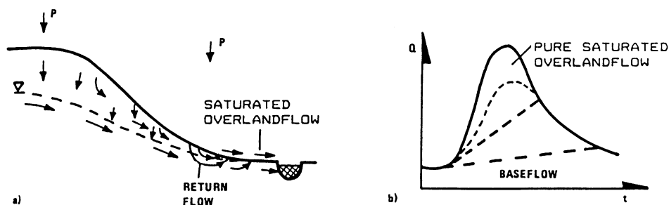
Fig. 1. Illustration of the dynamic response area model. a) Slope profile showing runoff processes. b) Typical hydrogram with different separation lines.
