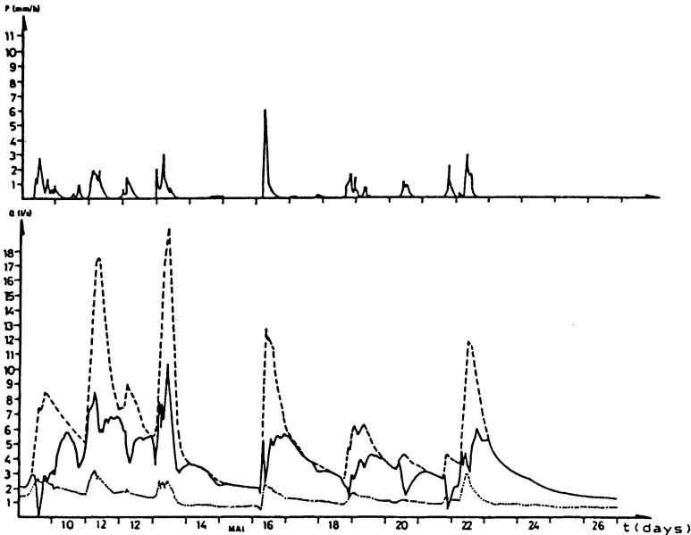
Fig. 6. Examples of hydrograph separation using two different methods, i.e. Eq. (1) and chemical conductivity. Precipitation and stream discharge data during the spring 1983 were used.
