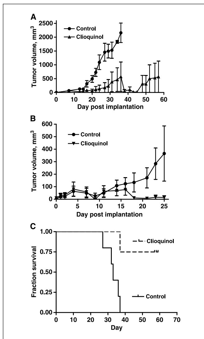
Figure 1. Effects of clioquinol on tumor growth in nude mice. Raji and A2780 cells were injected s.c. into the flanks of 5-week-old female nude mice. Clioquinol (28 mg/kg) was given i.p. 5 days a week, starting on day 8 after implanting. Tumor volume was calculated and expressed as cubic millimeters (mean \pm SE; control group, n = 4 ; clioquinol group, n = 5 ). A, inhibition of tumor growth of A2780 cells in nude mice. B, inhibition of tumor growth of Raji cells in nude mice. C, survival curve of A2780 cell-implanted mice.
