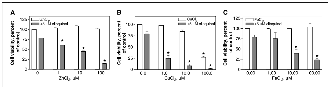
Figure 4. Addition of metals enhances clioquinol cytotoxicity in Raji cells. Cells were treated with \text{ZnCl}_2 , \text{CuCl}_2 , and \text{FeCl}_2 alone or premixed with 5 \mu\text{mol/L} clioquinol. After 72 hours of incubation, cell viability was determined using the MTS assay. Data (mean \pm SE, n = 3 ) are expressed as a percentage of untreated control cells. *, P < 0.05 , compared with control cells, using one-way ANOVA followed by Dunnett analysis.
