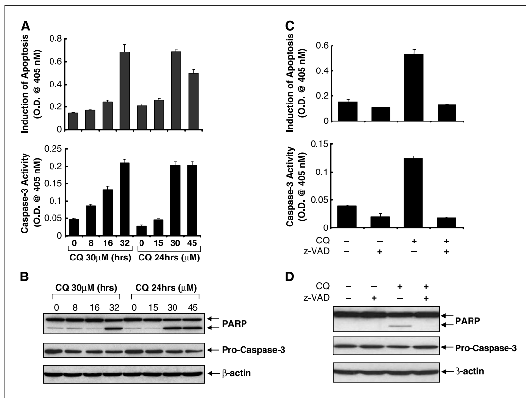
Figure 2. Clioquinol induces apoptosis in Raji cells through caspase-dependent mechanism. A , induction of apoptosis and caspase-3 activation by clioquinol (CQ). Raji cells were plated in 75-mm 2 flasks at 3 \times 10^6 cells per flask and treated with 30 \mu\text{mol/L} clioquinol for indicated time points or 24 hours with clioquinol for indicated concentrations. Cell lysates were prepared and subjected to apoptosis ELISA ( top ) and caspase-3 activity assay ( bottom ). B , an equal amount of protein for each sample as prepared in ( A ) was resolved by 8% SDS-PAGE followed by Western blot analysis with specific antibodies directed against PARP (BIOMOL Research Laboratories Inc., Plymouth Meeting, PA), caspase-3 (clone 19, monoclonal antibody, Transduction Laboratories, Lexington, KY), or \beta -actin (Sigma). C , abrogation of clioquinol-induced apoptosis and caspase-3 activation by caspase-specific inhibitor. Raji cells were plated in 75-mm 2 flasks at 3 \times 10^6 cells per flask and treated for 24 hours with either 30 \mu\text{mol/L} clioquinol or caspase pan-inhibitor z-VAD-fmk (Calbiochem Corp., San Diego, CA) alone or in combination of clioquinol and z-VAD-fmk. Cell lysates were prepared and subjected to apoptosis ELISA ( top ) and caspase-3 activity assay ( bottom ). D , an equal amount of protein for each sample as prepared in ( C ) was resolved by 8% SDS-PAGE, followed by Western blot analysis with specific antibodies directed against PARP, caspase-3, or \beta -actin. A and C , data (mean \pm SE, n = 3 ) are expressed as actual readings. B and D are representative of three independent experiments.
