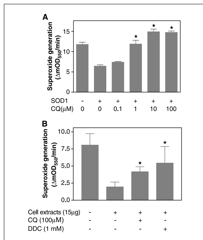
Figure 3. Effects of clioquinol on SOD1 activity. SOD1 activity was assayed with the xanthine oxidase/cytochrome C method as described in Materials and Methods. One unit of purified bovine erythrocyte SOD1 and 15 \mu\text{g} cellular extracts were used for the assay. A , clioquinol inhibits SOD1 activity in a concentration-dependent manner. B , clioquinol (100 \mu\text{mol/L} ) and diethyldithiocarbamate (DDC, 1 mmol/L) inhibit SOD1 activity in Raji cells after 6 hours' treatment. Data (mean \pm SE) are obtained from four to six independent experiments. *, P < 0.05 , compared with SOD1 activity control (second bar), using one-way ANOVA followed by Bonferroni analysis.
