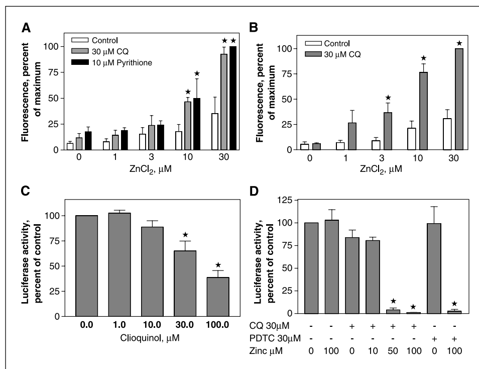
Figure 6. Effects of clioquinol on zinc uptake and NF \kappa B activity. A , A2780 cells were treated with 30 \mu M/L clioquinol and 10 \mu M/L pyrithione for 1 hour in the presence of various ZnCl 2 concentrations. B , Raji cells were treated with 30 \mu M/L clioquinol for 1 hour in the presence of various ZnCl 2 concentrations. The FluoZin-3 probe (3 \mu M/L) was then added to A2780 or Raji cells. After 30 minutes of incubation, cells were washed with fresh RPMI 1640 twice and kept in the incubator for another 30 minutes. The fluorescence was recorded at 485/535 nm (excitation/emission), using a Wallac 1420 Multilabel Counter. A and B , data (mean \pm SE, n = 3 ) are expressed as a percentage of maximum fluorescence detected. C , A2780 cells were treated with clioquinol for 4 hours at indicated concentrations. D , A2780 cells were treated with 30 \mu M/L clioquinol for 1 hour in the presence of various ZnCl 2 concentrations or with 30 \mu M/L pyrrolidine dithiocarbamate (PDTC) for 1 hour in the presence of 100 \mu M/L ZnCl 2 . Cell lysates were prepared and luciferase activity assayed as described in Materials and Methods. C and D , data (mean \pm SE, n = 3 ) are expressed as percentages of untreated control cells. *, P < 0.05 , compared with control cells, using one-way ANOVA followed by Dunnett analysis.
