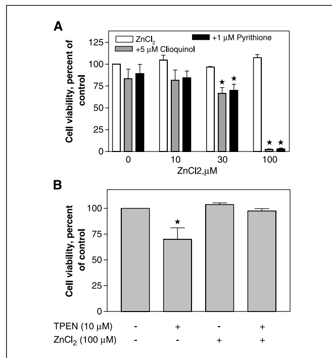
Figure 5. Effects of zinc-binding compounds on the viability of Raji cells. A, cells were grown in RPMI 1640 with supplements and treated with 5 \mu\text{mol/L} clioquinol or 1 \mu\text{mol/L} pyrithione for 72 hours in the presence of 10, 30, or 100 \mu\text{mol/L} \text{ZnCl}_2 . B, cells were treated with 10 \mu\text{mol/L} TPEN and 100 \mu\text{mol/L} \text{ZnCl}_2 for 72 hours. Cell viability was analyzed with the MTS assay. Data (mean \pm SE, n = 3 ) are expressed as a percentage of untreated control cells. *, P < 0.05 , compared with control cells, using one-way ANOVA followed by Dunnett analysis.
