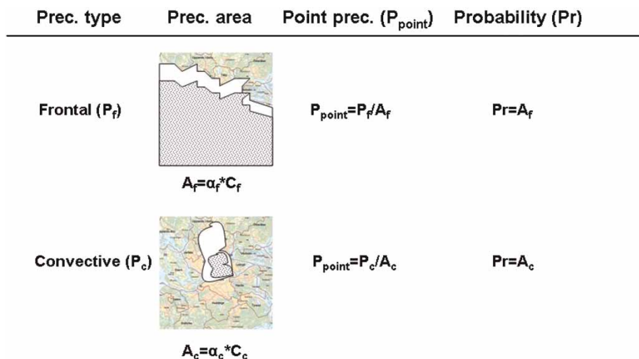
Figure 1 | Schematic of the stochastic downscaling scheme.
