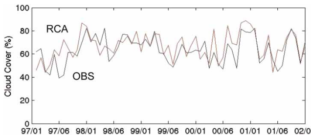
Figure 4 | Monthly total cloud cover in Stockholm as observed (OBS) and as simulated by RCA3 (RCA).
