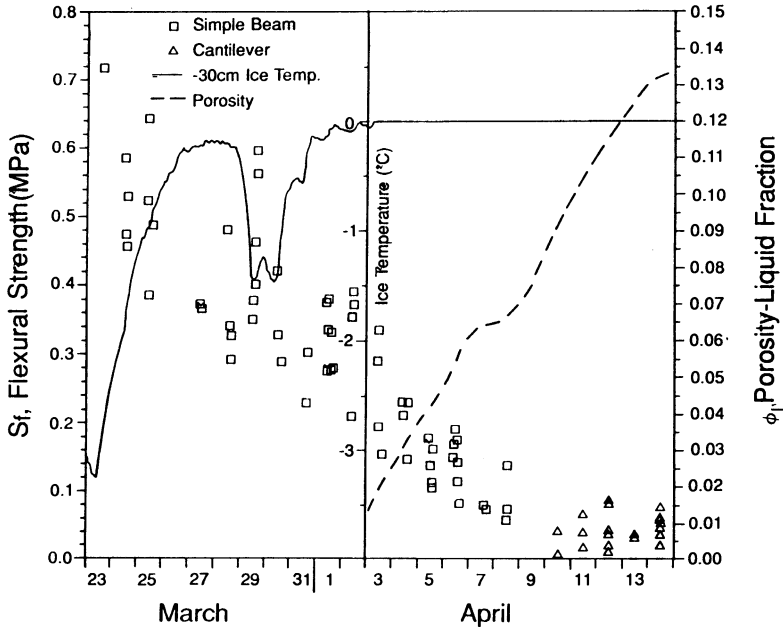
Fig. 4. Flexural strength, ice temperature and porosity.
