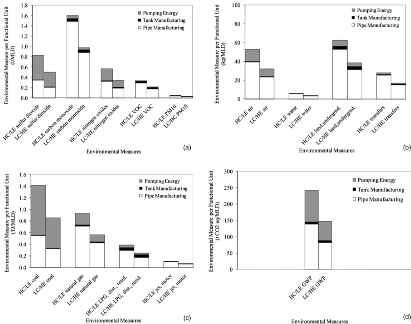
Figure 3 | Normalized environmental measures for the 'High cost/low energy' and 'Low cost/high energy' solutions with PVC pipe material.
