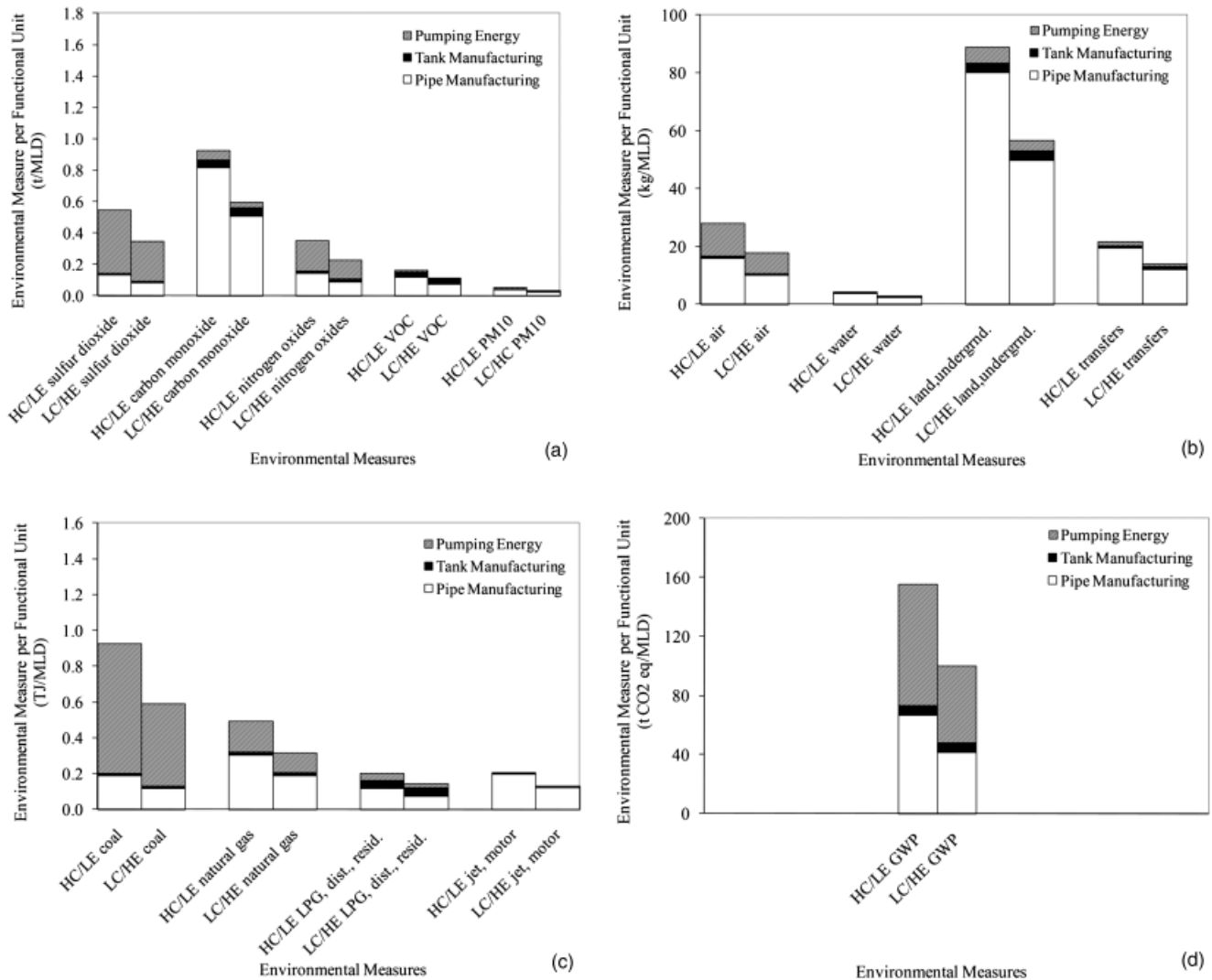
Figure 2 | Normalized environmental measures for the 'High cost/low energy' and 'Low cost/high energy' solutions with ductile iron (DI) pipe material.
