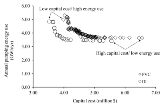
Figure 1 | Pareto-optimal fronts for capital cost versus annual pumping energy use for PVC and ductile iron (DI) pipe materials.
