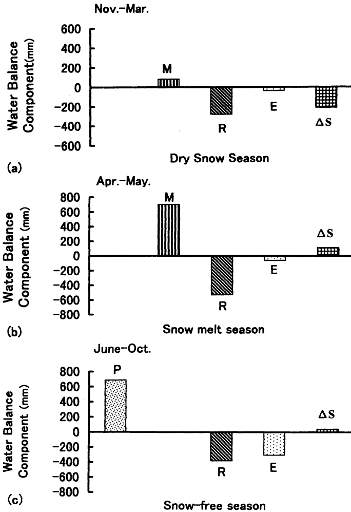
Fig. 10. Water balance at three different periods P : precipitation, R : runoff, E : evaporation, \Delta S : change of ground water storage, (a):dry snow season, (b):snowmelt season (c):snow-free season
