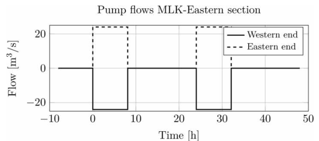
Figure 4 | Pump flows.
