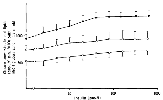
FIGURE 4. Lipogenesis at 37°C of fat cells as estimated by conversion of D-U-[ 14 C]glucose to total lipids at a glucose concentration of 0.5 mmol/L. Adipocytes from 10 nonpregnant normal women (●), 8 pregnant normal women (○), and 9 pregnant insulin-dependent diabetic women (□). Results are mean ± SEM.
