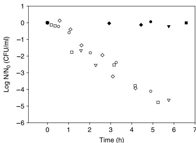
Figure 2 | Rate and reproducibility of inactivation of E. coli irradiated in FCRW on four separate dates. All trials were performed in quartz tubes. Open symbols: irradiated tubes; closed symbols: dark controls.
