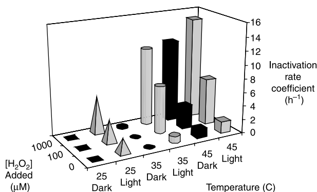
Figure 7 | Inactivation rate coefficient ( k ) versus temperature and [H_2O_2] added for E. coli K12 irradiated in FCRW in a temperature controlled batch reactor. Initial E. coli concentrations were between 2 \times 10^5 and 3 \times 10^6 CFU/ml in all experiments; experiments ranged in duration from 2 to 6.5 h.
