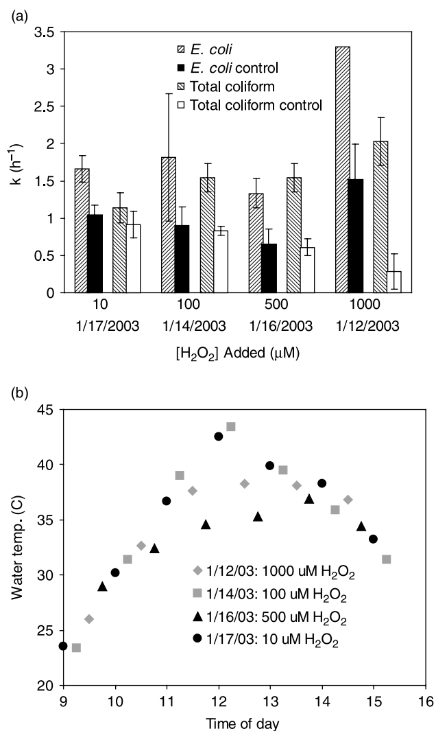
Figure 5 | (a) Inactivation rate coefficients ( k ) for indigenous E. coli and total coliforms in Haiti surface water samples exposed to natural sunlight with and without added hydrogen peroxide on different days. 1/16/2003 was cloudy while the other days were mostly sunny. No detectable E. coli remained after 1 h for the 1000 μM H 2 O 2 added trial on 1/12/2003; therefore the minimum inactivation rate required to produce <1 detectable colony at 1 h is shown for this condition and an error bar could not be calculated. (b) Water temperature vs. time of day for each of the inactivation experiments plotted in (a).
