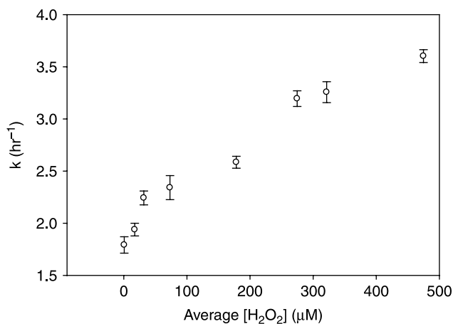
Figure 3 | Inactivation rate coefficients ( k ) for E. coli K12 vs. average hydrogen peroxide concentration. A linear regression of the data points gives a slope of 0.0037 \text{h}^{-1}\mu\text{M}^{-1} with a y-intercept of 2.0 and an r^2 value of 0.95.
