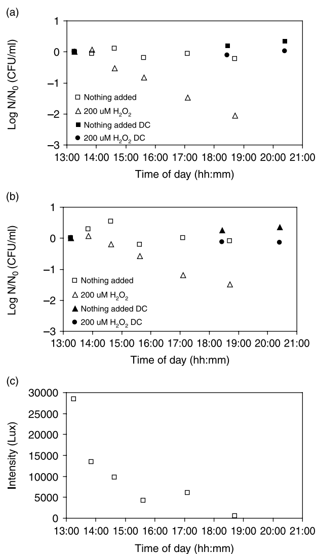
Figure 6 | Inactivation of naturally present (a) E. coli and (b) total coliforms vs. time in Bombay ditchwater with nothing or 200 μM H 2 O 2 added. DC = dark control. Initial concentrations of both E. coli and total coliforms were on the order of 10 3 CFU/ml (c).
