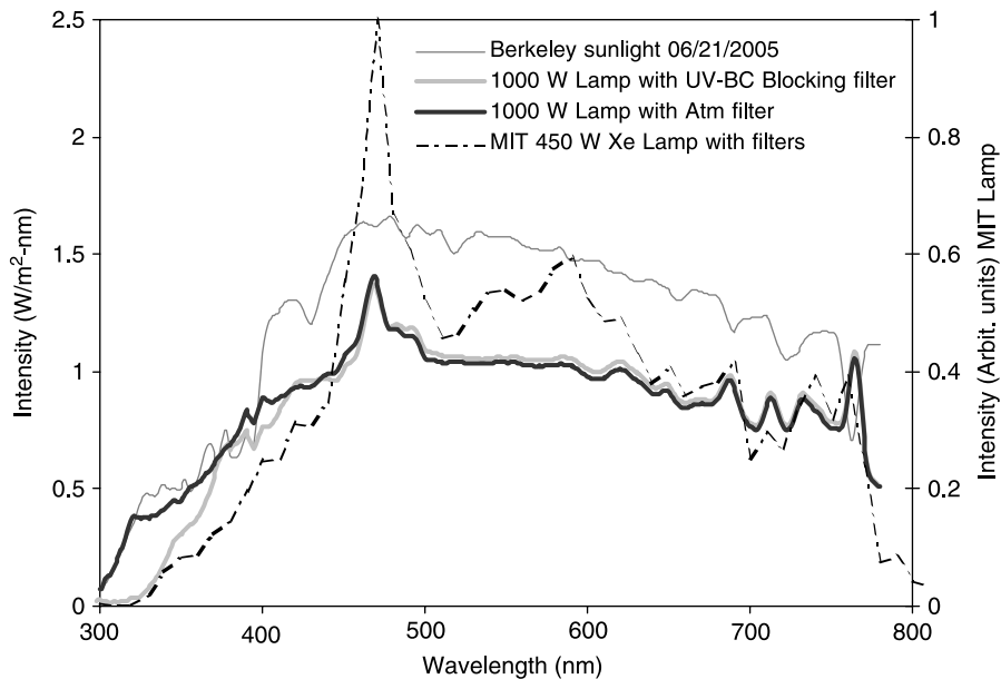
Figure 1 | Irradiance spectra for sunlight, UCB 1000W solar simulator with two different filter sets, and MIT 450W lamp with filters. Sunlight and UCB spectra were measured directly, whereas the spectrum shown for MIT was calculated from the manufacturer's published 1000W lamp spectrum and corrected for the filters used.
