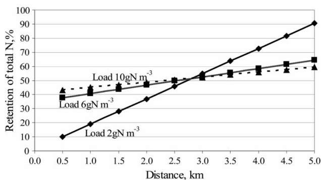
Figure 5 | The dependency of total N retention in stream water on different loads, from pollution source and distance downstream.
