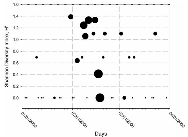
Figure 5 | Daily Shannon diversity index for Utility A during earth/musty outbreak. The size of the point indicates the total number of complaints that day. Large points with low diversity indicate potential water quality problems.
