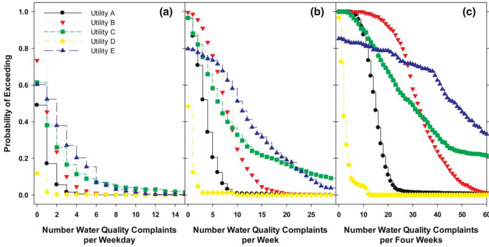
Figure 3 | Exceedance plots for the total number of water quality complaints that occurred per day, week (7 day), and month (28 days).
