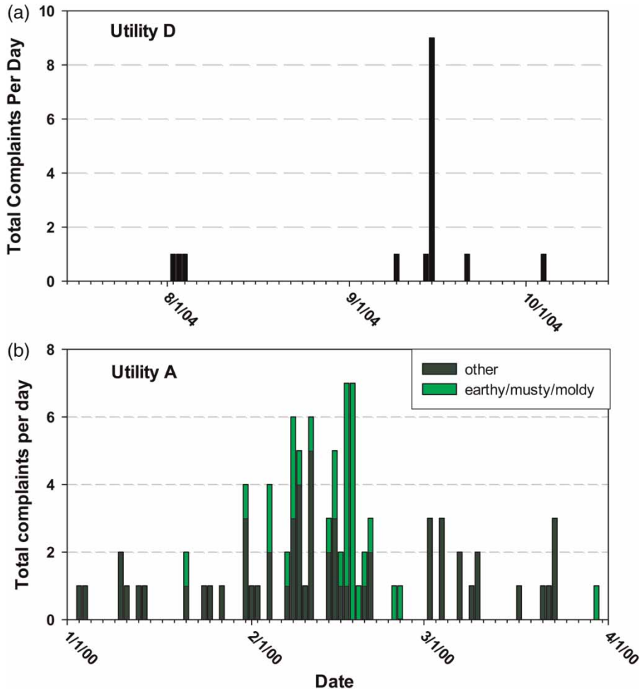
Figure 2 | Example water quality events found through customer complaints for (a) Utility D and (b) Utility A. (a) Represents an example of a very sudden short term event. (b) Represents a gradually worsening earthy-musty event above normal background complaint levels.
