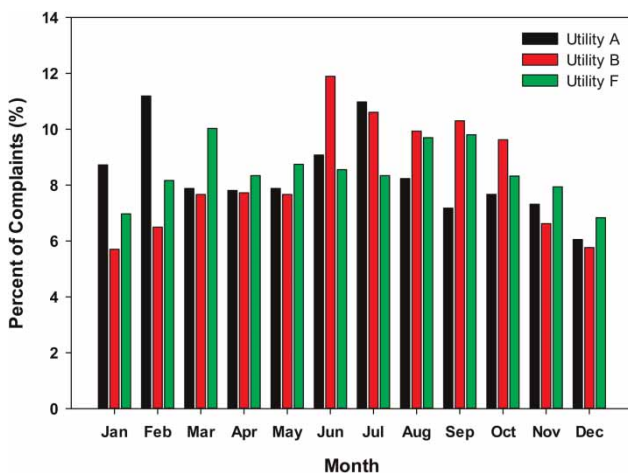
Figure 1 | Percentage of complaints by month.
