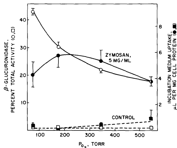
FIGURE 3 Phagocytosis and \beta -glucuronidase release under varying P_{O_2} . Leukocytes were incubated with (circles) or without (squares) zymosan, 5 mg/ml, for 1 h. A trace amount of [ ^{14}C ]inulin was present in all tubes. Phagocytosis (solid symbols) was estimated by the uptake of extracellular water into the cell pellets, using [ ^{14}C ]inulin as a marker. \beta -Glucuronidase activity in incubation media was measured as an index of lysosomal enzyme release. See Fig. 1 and text for further details.
