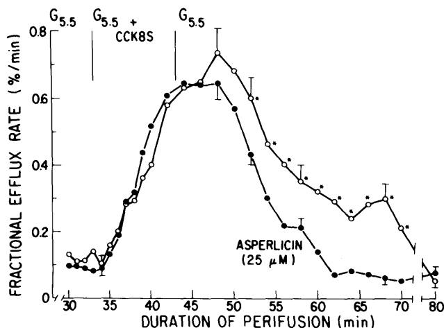
FIG. 5. Sustained activation of ^3\text{H} efflux induced by brief CCK-8S exposure. After 2-h labeling period in [ ^3\text{H} ]inositol, islets were perfused for 30 min with 5.5 mM glucose (G) alone. They were then stimulated with 200 nM CCK-8S for 10 min followed by 40 min perfusion with 5.5 mM glucose \pm 25 \mu\text{M} asperlicin. CCK-8S-induced efflux of ^3\text{H} from these islets remained significantly ( P < .05 ) elevated above prestimulatory rates for \sim 30 min after CCK-8S removal from medium ( n = 6 for each condition). Inclusion of asperlicin during final 40-min period significantly ( *P < .05 ) reduced this persistent increase in ^3\text{H} efflux.
