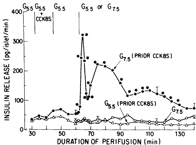
FIG. 1. CCK-8S-induced sensitization to glucose stimulation. Groups of islets were collagenase isolated and perfused with 5.5 mM glucose (G) for 30 min to establish basal, stable rates of release. Medium was then supplemented with 200 nM CCK-8S for 10 min. After a further 20-min perfusion in CCK-8S-free medium, these islets were then stimulated for 80 min with 7.5 mM glucose. Secretory response of control islets, not previously exposed to CCK-8S, is depicted as well as the response of islets exposed to CCK-8S for 10 min but maintained with 5.5 mM glucose for rest of perfusion ( n = at least 4 for each condition). *Significant differences ( P < .05 ) in release rates between control islet response to 7.5 mM glucose versus those previously exposed to CCK-8S.
