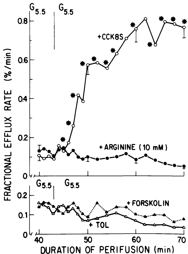
Fig. 4. Fractional efflux rates of ^3\text{H} from islets prelabeled with [ ^3\text{H} ]inositol. Islets were incubated for 2 h in [ ^3\text{H} ]inositol to label inositol-containing lipids. After being washed with 5 ml of nonradioactive medium, islets were perfused for 40 min with 5.5 mM glucose (G) alone. They were then stimulated with 200 nM CCK-8S, 10 mM arginine, 25 \mu M tolbutamide (TOL), or 1.0 \mu M forskolin ( n = at least 3 for each condition). Efflux rates of ^3\text{H} were calculated according to Borle et al. (12). Only addition of CCK-8S to these islets significantly increased ( *P < .05 ) efflux of [ ^3\text{H} ]inositol, an index of accelerated phosphoinositide turnover, above prestimulatory values.
