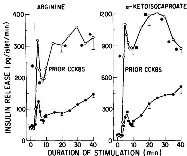
FIG. 2. Prior CCK-8S exposure sensitizes islets to arginine and \alpha -ketoisocaproate. Left panel: groups of islets were perfused for 30 min with 5.5 mM glucose. For an additional 10 min, 200 nM CCK-8S was included in medium. After 10 min perfusion in CCK-8S-free medium, islets were provoked with 10 mM arginine for 40 min in continued presence of 5.5 mM glucose. Response to control islets (untreated with CCK-8S) is also shown ( n = 3 for each condition). Right panel: similar to protocol described above, islets were provoked with 10 mM \alpha -ketoisocaproate for 40 min (in continued presence of 5.5 mM glucose) after prior exposure to 200 nM CCK-8S for 10 min. Control response from untreated islets is also shown ( n = 3 for each condition). *Selected time points were analyzed for significance ( P < .05 ).
