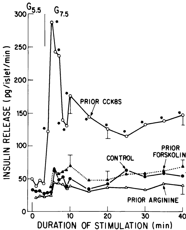
Fig. 3. Prior exposure to arginine or forskolin does not sensitize islets to 7.5 mM glucose (G). Similar to protocol described in Fig. 2, islets were exposed to 10 mM arginine, 1.0 \mu M forskolin, or 200 nM CCK-8S for 10 min. Although not depicted, release rates (in continued presence of 5.5 mM glucose) in response to arginine, forskolin, tolbutamide, or CCK-8S averaged 96 \pm 7 , 132 \pm 23 , 127 \pm 15 , and 57 \pm 6 \text{pg} \cdot \text{islet}^{-1} \cdot \text{min}^{-1} (means \pm SE), respectively, during the final 5 min of exposure to these agents. This compares with control release rates of 31 \pm 4 \text{pg} \cdot \text{islet}^{-1} \cdot \text{min}^{-1} during same period. After a further 10-min perfusion with 5.5 mM glucose alone, islets were stimulated for 40 min with 7.5 mM glucose. Response of control islets is also shown. Arginine, forskolin, and tolbutamide did not sensitize islets to 7.5 mM glucose ( n = at least 4 for each; not shown). *Significant difference ( P < .05 ) from control untreated islet response.
