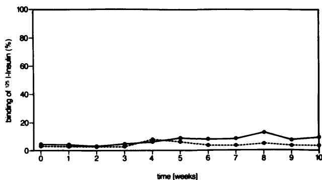
FIG. 4. Binding of 125 I-insulin to sera from 5 pigs immunized with insulin taken from pump eluates in vitro (dashed line) and insulin unexposed to programmable implantable medication system (solid line). See text for details.
