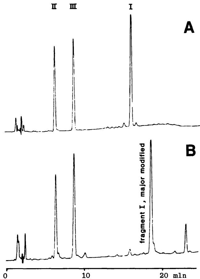
FIG. 3. A , Staphylococcus aureus protease V8 fingerprint HPLC analysis of human insulin major modification product (MMP) showing 3 major fragments. B , S. aureus protease V8 fingerprint HPLC analysis of Hoe 21 PH showing identical patterns for MMP from human insulin, with the exception of fragment I, which is eluted significantly later. See ref. 21 for details.
