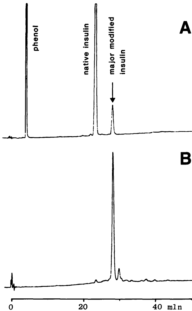
FIG. 2. A , typical preparative HPLC tracing of insulin from programmable implantable medication system pump eluate in vitro (see text), showing elution of phenol, native insulin, and major modified product of insulin. B , the isolated peak from major modified product of insulin, showing that native insulin was practically absent, whereas desamido-A21 derivative of major modified product, formed during HPLC preparation, is present.
