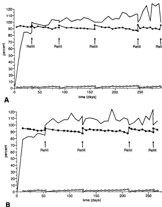
FIG. 1. In vitro tests of Hoe 21 PH U-400 insulin stability in 2 programmable implantable medication systems (A and B). Samples collected from pump eluates were assayed by HPLC. Refills were performed at times indicated by arrows. Solid line, total insulin concentration as percent of external insulin standard; ●, percent of total insulin assayed as native insulin by HPLC; ○, percent of total insulin assayed as major modification product (see text).
