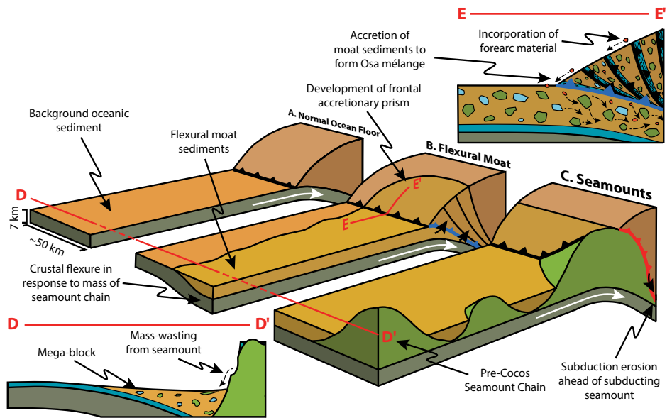
Figure 3. Conceptual model of frontal accretion of seamount moat sediments adjacent to subduction erosion by subduction of seamount. White arrows indicate convergence direction. A: Subduction of oceanic plate under conditions normal for this margin. B: Subduction of moat leading to increased accretion and development of frontal accretionary prism, even in otherwise non-accretionary subduction zones. This is the setting in which Osa mélangé formed. Blue ticked line shows subduction accretion. C: Subduction of seamount (green) leading to increased local subduction erosion of upper plate (e.g., Ranero and von Huene, 2000; Vannucchi et al., 2016). Material eroded from base of forearc may be mixed with subducted moat sediments and reaccreted. Red ticked line shows subduction erosion. Insets show cross-sections beneath lines D–D' and E–E'; D–D' shows mass wasting from volcanic edifice into moat; E–E' shows accretion of flexural moat into localized accretionary prism (see B) and mixing with upper-plate blocks.
