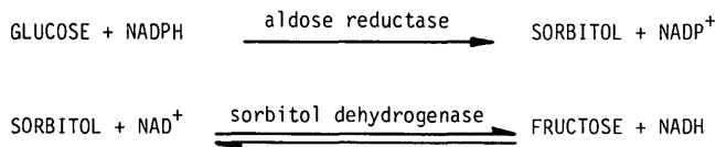
FIG. 1. Schema of polyol pathway.
