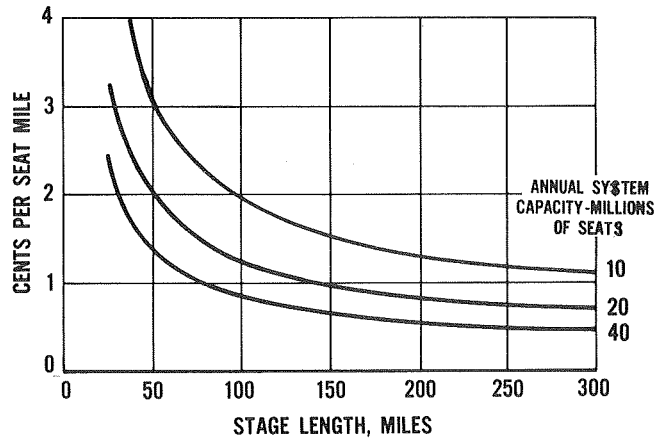
Fig. 15 Indirect operating costs
