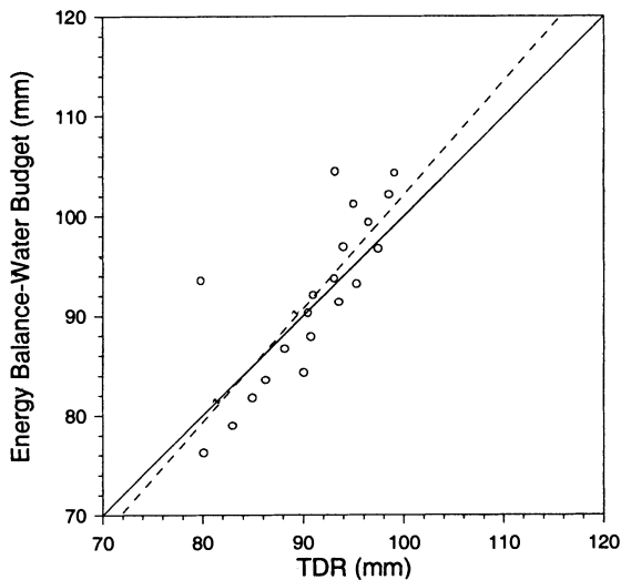
Fig.8. Comparing daily soil moisture from the EBWB with TDR measurements at Kendall during the summer rainy period (1990).
