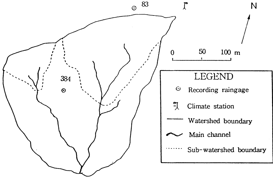
Fig.2. The locations of measurement stations at Lucky Hills watershed.
