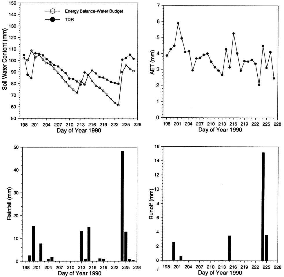
Fig.5. Water balance during the summer rainy period (1990) at Lucky Hills watershed.
