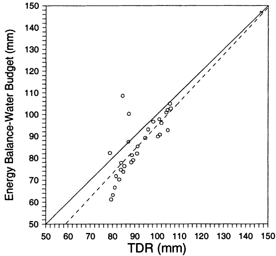
Fig.7. Comparing daily soil moisture from the EBWB with TDR measurements at Lucky Hills during the summer rainy period (1990).
