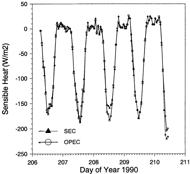
Fig.4. Comparison of OPEC sensible heat and SEC sensible heat at Walnut Gulch.
