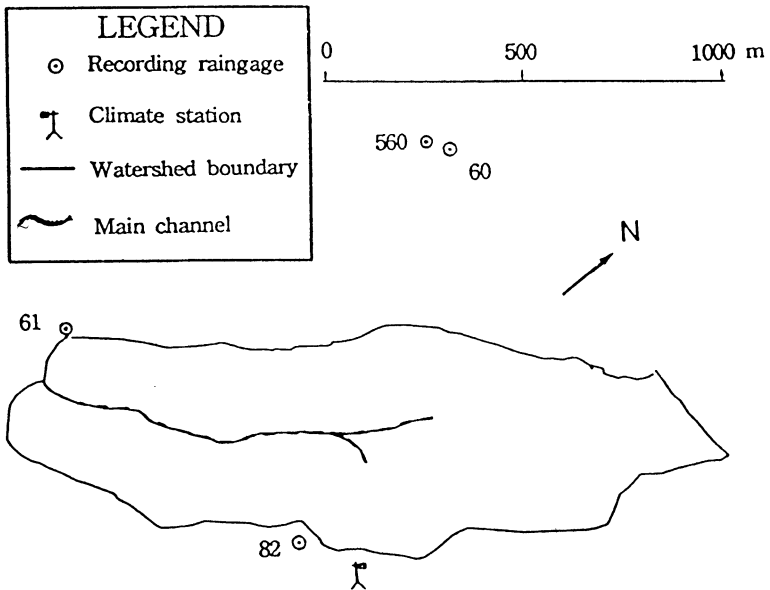
Fig.3. The locations of measurement stations at Kendall watershed.
