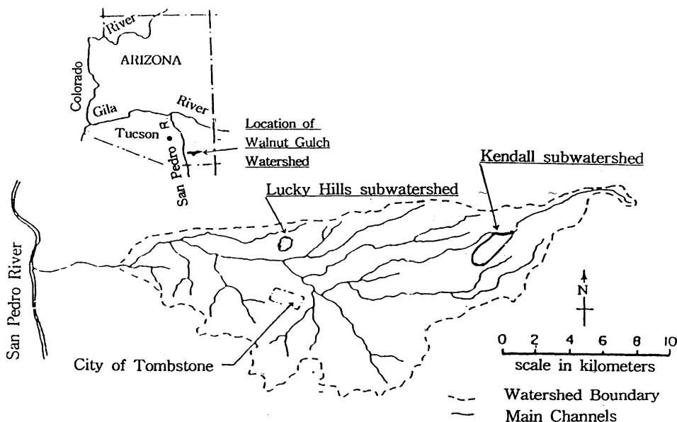
Fig.1. USDA-ARS Walnut Gulch experimental watershed location map.
