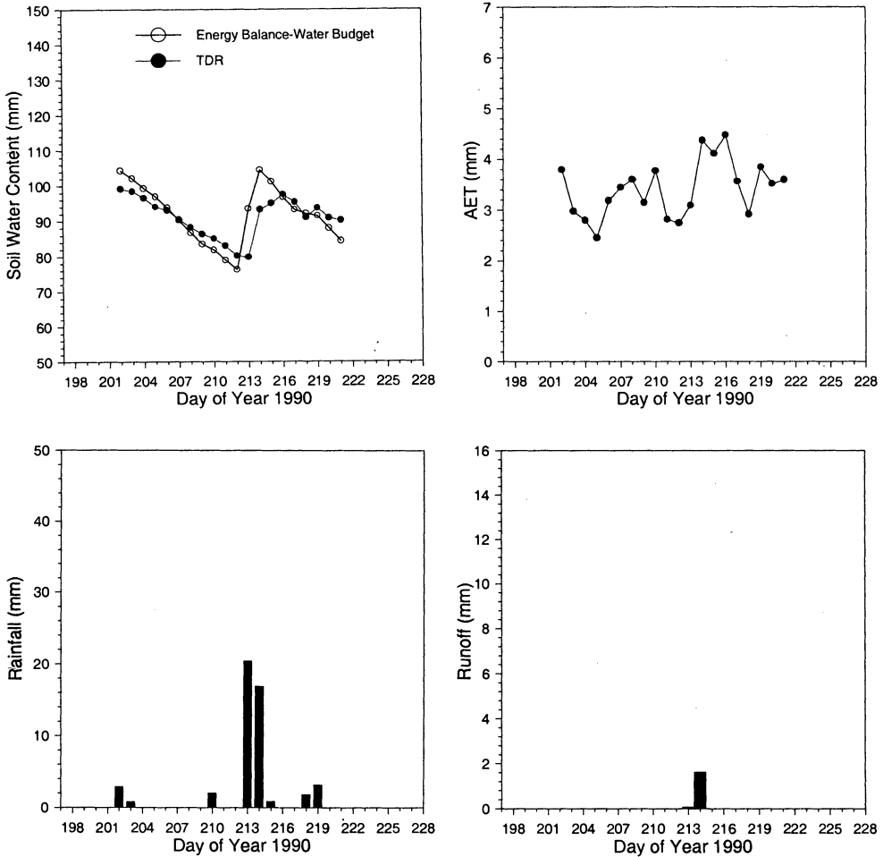
Fig.6. Water balance during the summer rainy period (1990) at Kendall watershed.
