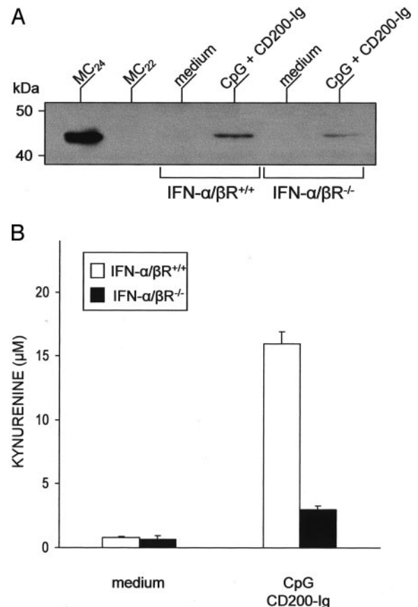
FIGURE 6. Failure of CD200-Ig to induce IDO expression and function in pDCs from IFN- \alpha \beta R -/- mice. A , IDO expression by immunoblot analysis. pDC from wild-type (IFN- \alpha \beta R +/+ ) and knockout (IFN- \alpha \beta R -/- ) mice were treated in vitro with CD200-Ig plus CpG, MC 24 , and MC 22 transfectants representing the positive and negative controls, respectively. Loading controls (not shown) consisted of samples reprobated with \beta -actin-specific Ab. One experiment of two. B , Functional IDO activity in response to CD200-Ig plus CpG was measured in terms of ability to metabolize tryptophan to kynurenine, using the same mice as above as a source of pDCs. Kynurenine levels in supernatants are means \pm SD of triplicate samples in one of three experiments.
