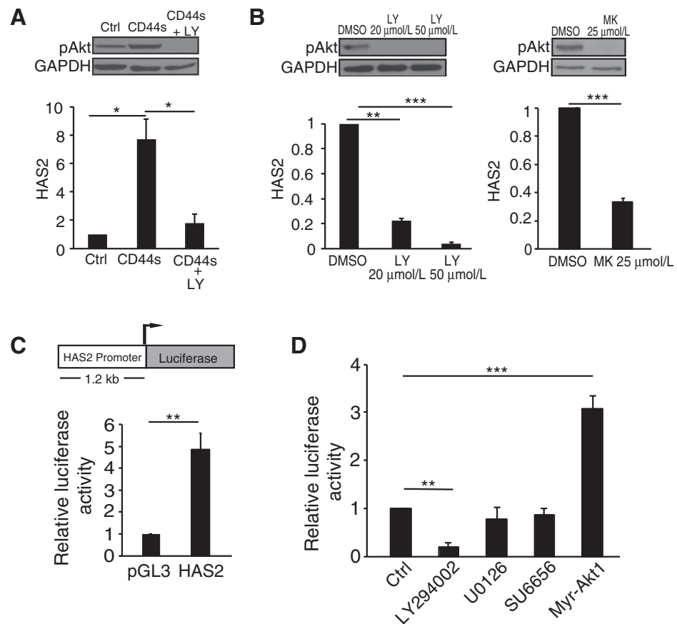
Figure 3. CD44s-mediated HAS2 transcription is dependent on Akt signaling. A , qRT-PCR analysis showing that CD44s-dependent HAS2 upregulation is abolished by the PI3K/Akt inhibitor LY-294002 (LY; 20 \mu mol/L). Control and CD44s-overexpressing Mes10A cells were collected 20 hours after treatment. Immunoblot images on the top plot showing that LY-294002 effectively inhibited Akt activity. B , qRT-PCR analysis showing that inhibition of Akt signaling by LY-294002 (LY; 20 \mu mol/L and 50 \mu mol/L, left) or MK-2206 (MK; 25 \mu mol/L, right) suppressed expression of endogenous HAS2 in LM2 cells. Cells were treated for 20 hours. Immunoblot images on the top plot showing that LY-294002 and MK-2206 inhibited Akt activity in LM2 cells. C , Top, a schematic of the HAS2 promoter-driven luciferase reporter construct. Bottom, relative luciferase activity in 293FT cells transfected with the HAS2 luciferase reporter construct. D , Relative luciferase activity in 293FT cells transfected with the HAS2 luciferase reporter construct and treated with LY-294002 (20 \mu mol/L), U0126 (25 \mu mol/L), SU6656 (5 \mu mol/L), or cotransfected with Myr-Akt1. For each luciferase activity assay, ratios of firefly-to- Renilla luciferase activities were normalized to cells cotransfected with an empty vector control. Error bars, SD; n = 3 . *, P < 0.05 ; **, P < 0.01 ; ***, P < 0.001 .
