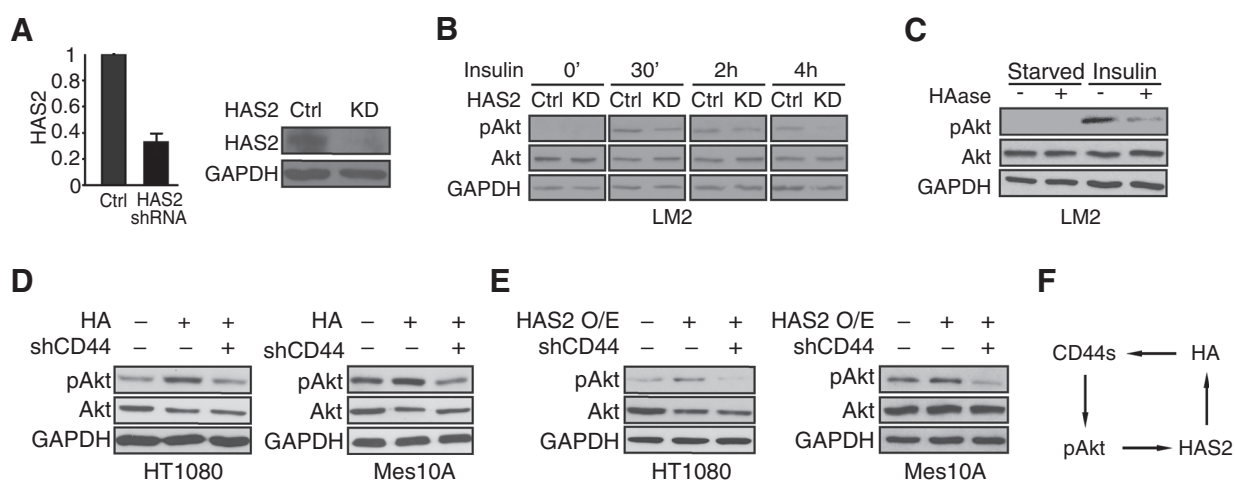
Figure 4. HAS2/HA promotes Akt activation in a CD44s-dependent manner. A , qRT-PCR and immunoblot analyses showing that HAS2 was silenced in HAS2 shRNA-expressing (KD) LM2 cells. Error bars, SD; n = 3 . B , Immunoblot analysis of pAkt levels showing that HAS2 knockdown inhibits Akt activity. Control and HAS2 knockdown LM2 cells were stimulated with insulin (10 \mu\text{g}/\text{mL} ) and collected at different time intervals. C , Immunoblot analysis of pAkt levels showing that HAase treatment impairs Akt phosphorylation. Control and HAase-treated (100 \mu\text{g}/\text{mL} , 6 hours) LM2 cells were stimulated with insulin (10 \mu\text{g}/\text{mL} ) and collected 30 minutes after stimulation. D , Immunoblot analysis of pAkt levels showing that HA stimulates Akt activation in a CD44-dependent manner. HT1080 and Mes10A cells were grown on HA-coated plates (0.5 mg/mL HA for HT1080; 0.1 mg/mL HA for Mes10A). HT1080 and Mes10A cells were collected 24 hours after plating on HA-coated plates. E , Immunoblot analysis of pAkt levels showing that CD44 is required for HAS2-promoted Akt activation. Control and HAS2-overexpressing HT1080 cells were cultured in regular media for 24 hours after plating and collected for immunoblot analysis. Control and HAS2-overexpressing Mes10A cells were starved overnight and stimulated with insulin (10 \mu\text{g}/\text{mL} , 30 min) before lysate collection. F , A model of a positive feedback loop, involving CD44s and HAS2/HA, that sustains Akt activation.
