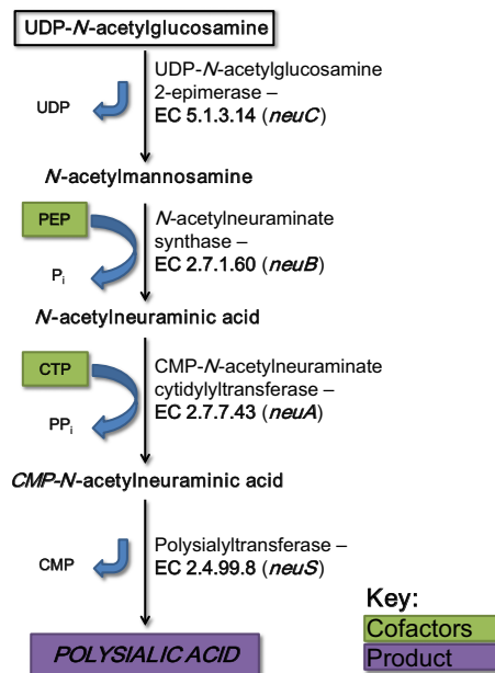
Fig. 6. Biosynthetic pathway for PSA production in Escherichia coli K1.
