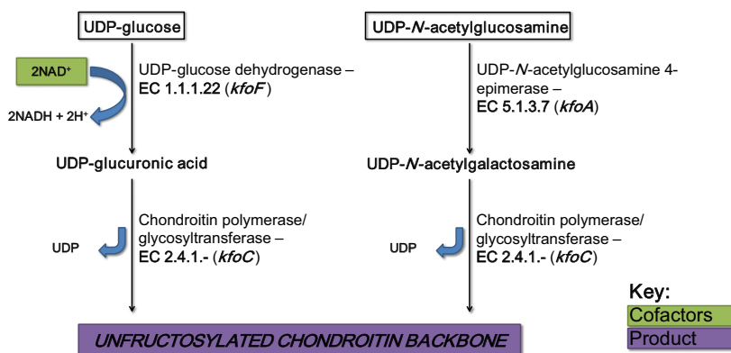
Fig. 7. Biosynthetic pathway for production of K4 CPS, chondroitin, in Escherichia coli K4.
