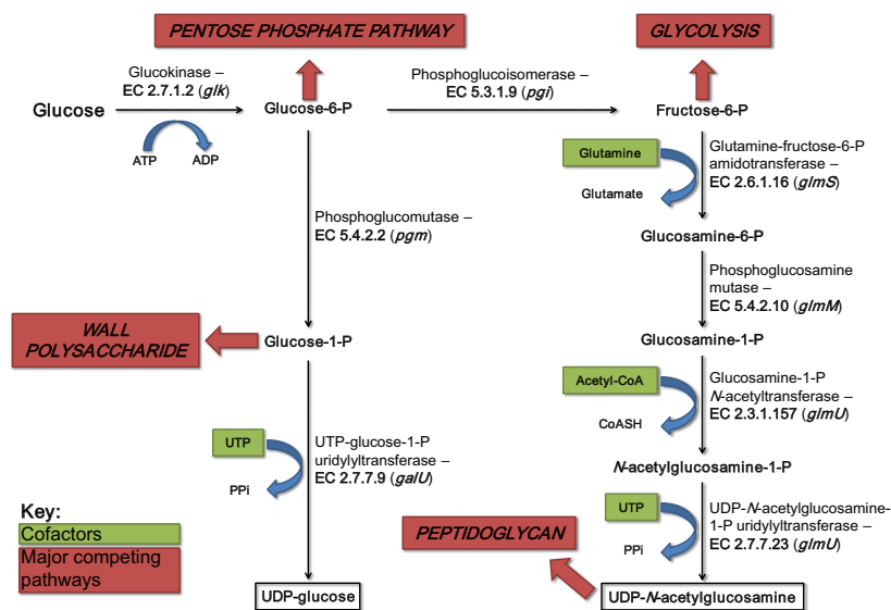
Fig. 5. Central biosynthetic pathway for CPS precursor production in Escherichia coli . This metabolic model is representative of early CPS biosynthesis for many bacteria, including those of interest in this review.
