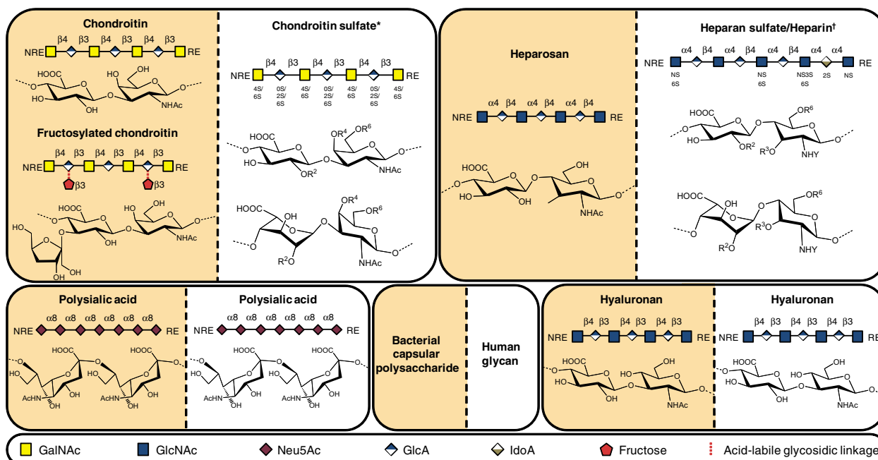
Fig. 3. Symbolic representations and chemical structures of glycans described in this review. Nonimmunogenic bacterial CPSs and structurally related animal glycans exhibited side-by-side to demonstrate similarity between backbones. In the case of chondroitin sulfate (CS) and heparan sulfate/heparin, bacterial CPS structures are identical to precursors of the mature human glycans depicted here. Of note, a related GAG known as dermatan sulfate also shares the unsulfated chondroitin backbone as a biosynthetic precursor, but, unlike CS, some glucuronic acid residues in the chain are epimerized to iduronic acid. CS type B possesses iduronic acid residues, so it is sometimes classified as dermatan sulfate. Conversely, HA and PSA structures are identical in microbial CPS and mature human glycans. * R^{2,4,6} = H or SO_3^- ; ^{\dagger}R^{2,3,6} = H or SO_3^- , Y = SO_3^- or Ac (Ac = COCH_3 ). Detailed disaccharide structures have been reported elsewhere (Sugahara & Mikami, 2007; Chang et al. , 2012b).
