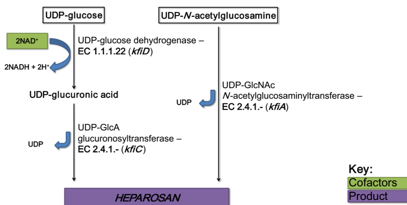
Fig. 8. Biosynthetic pathway for production of K5 CPS, heparosan, in Escherichia coli K5.
