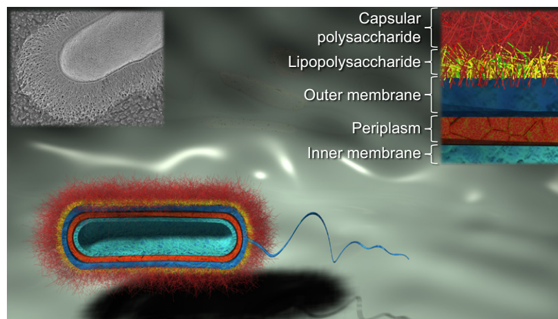
Fig. 1. Schematic cross-sectional representation of layers constituting the bacterial cell wall of a typical Gram-negative bacterium. The thick external CPS layer conceals the bacterium to prevent desiccation, bacteriophage infection, complement-mediated killing, and opsonophagocytosis. The black and white inset (top left) shows a quick-freeze, deep-etch scanning electron micrograph of the Gram-negative organism Bacteroides thetaiotaomicron (Martens et al. , 2009); this SEM image was originally published in The Journal of Biological Chemistry. Martens EC, Roth R, Heuser JE & Gordon JI. Cover image. J Biol Chem. 2009; 284 (27):cover. © the American Society for Biochemistry and Molecular Biology.
