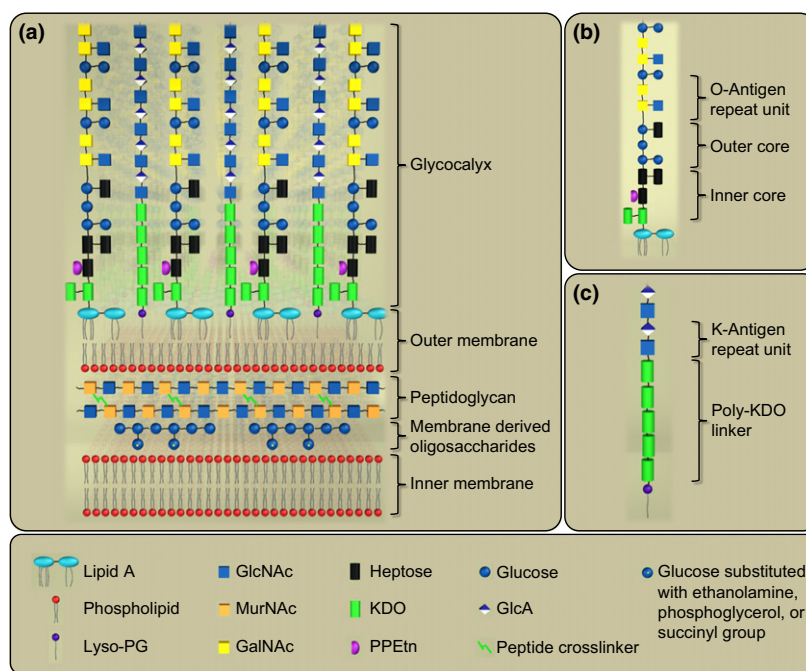
Fig. 2. Glycan-centric schematic of typical Gram-negative cell wall components. Membrane proteins and other cell wall constituents are neglected for simplicity. (a) Cell wall cross-section. (b) Lipopolysaccharide. (c) Capsular polysaccharide. Abbreviations are as follows: Lyso-PG = lyso-phosphatidylglycerol, GlcNAc = N -acetylglucosamine, MurNAc = N -acetylmuramic acid, GalNAc = N -acetylgalactosamine, KDO = 3-deoxy- D -mannooctulosonic acid, PPEtn = pyrophosphoethanolamine, GlcA = glucuronic acid.
