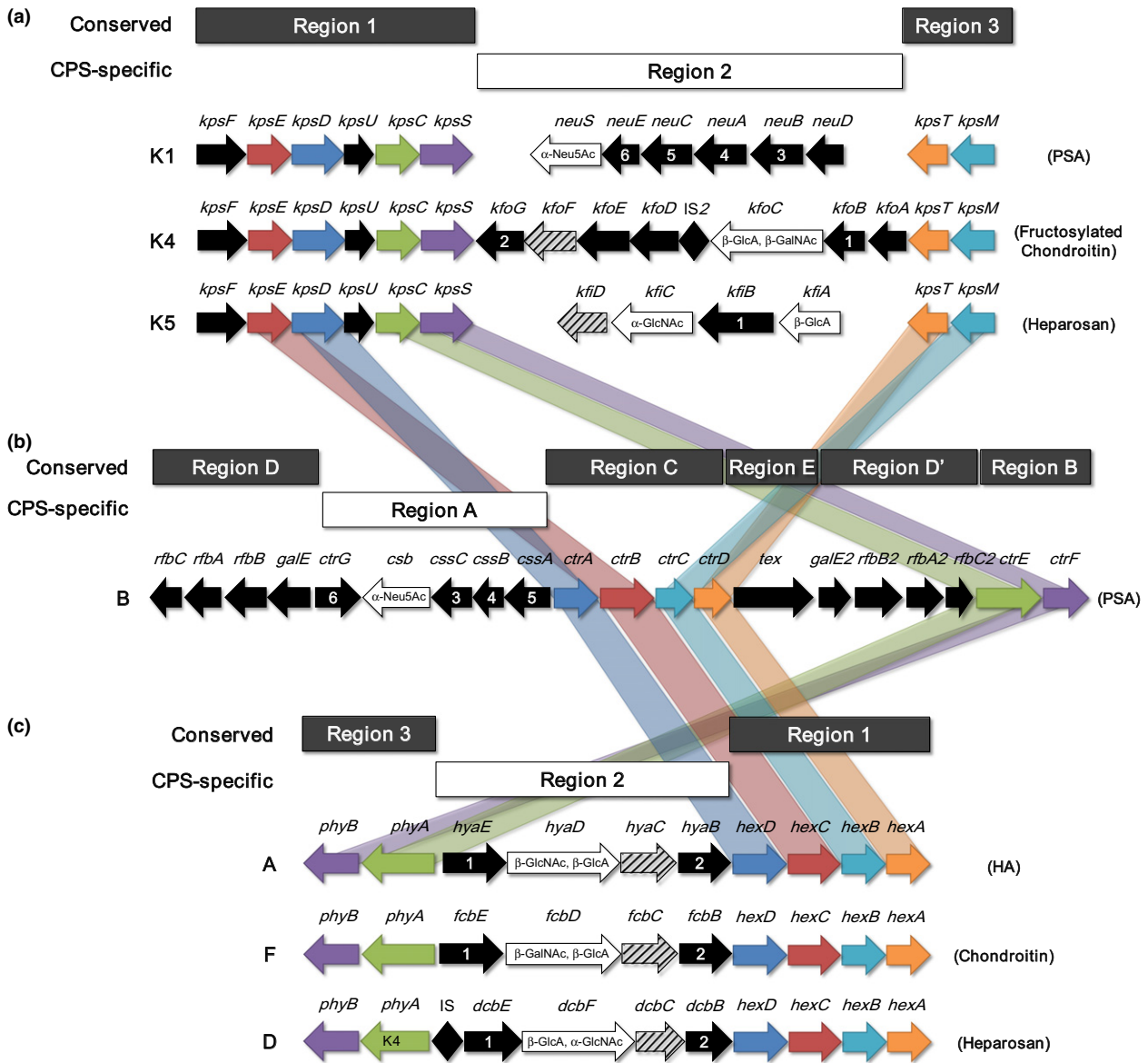
Fig. 4. CPS gene loci in Gram-negative bacteria expressing ABC-transporter-dependent CPS assembly pathways. (a) Gene loci encoding enzymes and transport proteins required for assembly of Group 2 Escherichia coli K-antigens K1 (polysialic acid), K4 (chondroitin), and K5 (heparosan). Genes encoded by Regions 1 and 3 are well conserved within Group 2 E. coli strains and encode enzymes required for CPS translocation across the cell wall, while Region 2 encodes CPS-specific glycosyltransferases and other biosynthetic enzymes. (b) Gene locus encoding proteins required for assembly of Neisseria meningitidis serogroup B CPS. Region A encodes CPS-specific biosynthetic enzymes and varies between serogroups, while Regions B–E are highly conserved in all N. meningitidis serogroups. Regions B and C encode CPS translocation proteins homologous to genes in Regions 1 and 3 of Group 2 E. coli , Regions D and D' encode LPS assembly genes, and Region E has no known function. (c) Gene loci encoding Pasteurella multocida type A, D, and F CPS biosynthetic and transport proteins. Regions 1 and 3 encode translocation genes whose functions are relatively well conserved in P. multocida , and Region 2 encodes CPS biosynthetic enzymes unique to the serotype specified. Homologous interspecies transport genes are color coded and connected by bands of matching colors. Genes encoding glycosyltransferases are illustrated as white arrows with black outline and glycosyltransferase activity denoted within (bifunctional glycosyltransferases are labeled as found in nature, with N-terminal domain displayed at 5' end of gene and C-terminal domain displayed at 3' end of gene). UDP-glucose dehydrogenase is frequently encoded in CPS-specific biosynthetic clusters and is indicated here with diagonal lines. Other genes with known and putative homologs are designated with matching numbers. Note: genes and operons are not drawn to scale.
