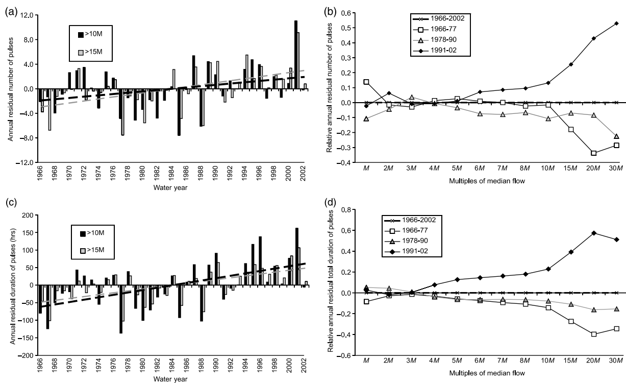
Figure 6 | Time series of (a) annual residual pulse number and (c) annual residual pulse duration above thresholds of 10M–15M, and relative annual residual (b) number of pulses and (d) duration of pulses for the range of thresholds and sub-periods. (Note: “Relative” means that average residuals have been normalized by the total number or duration of pulses (depending on the case) for each threshold for a better scaling and understanding of the magnitude of the changes).
