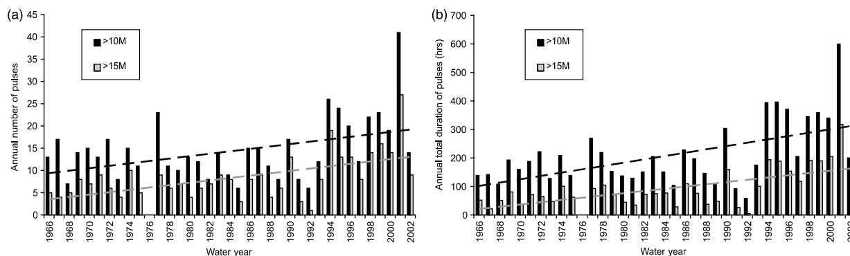
Figure 5 | (a) Time series of (left) annual number of pulses above thresholds of 10M (10 times the median flow) and 15M. (b) Annual total duration of pulses above thresholds of 10M and 15M.
