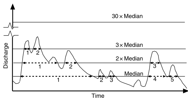
Figure 4 | Schematic definition diagram for pulse numbers and pulse duration (Archer 2000).
