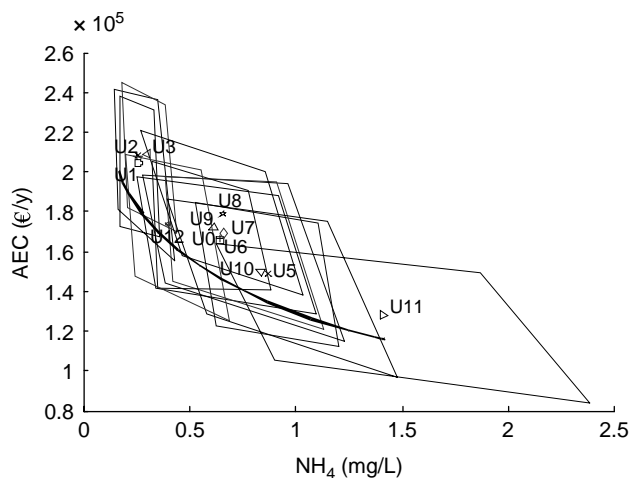
Figure 8 | \text{NH}_4 and AEC for LLAS upgrades in Continental climate; bold line: Pareto front.
