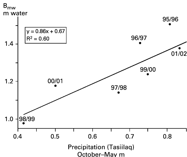
Figure 4 Relationship between the observed winter precipitation (October–May) in Tasiilaq and the measured winter balance at Mittivakkat Gletscher during the balance years 1995–2002
