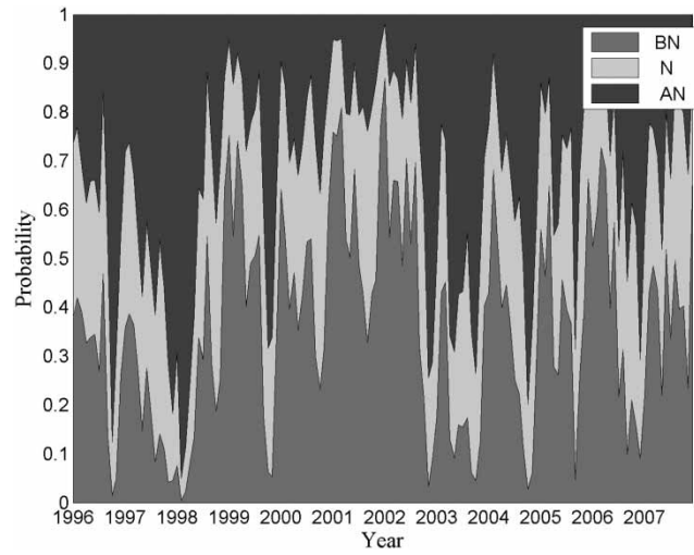
Figure 9 | Monthly probabilistic forecasts over the three categories for every month during the validation period.
