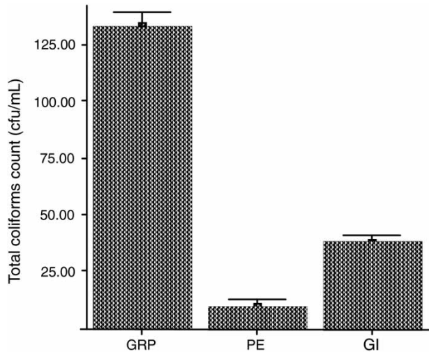
Figure 3 | Total coliform count of GRP, PE and GI tanks ( n = 40 replications/treatment).
