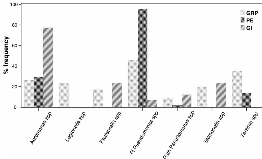
Figure 8 | Composition of microbial biofilms in GRP, PE and GI tanks; FI = fluorescent; Path = pathogenic.
