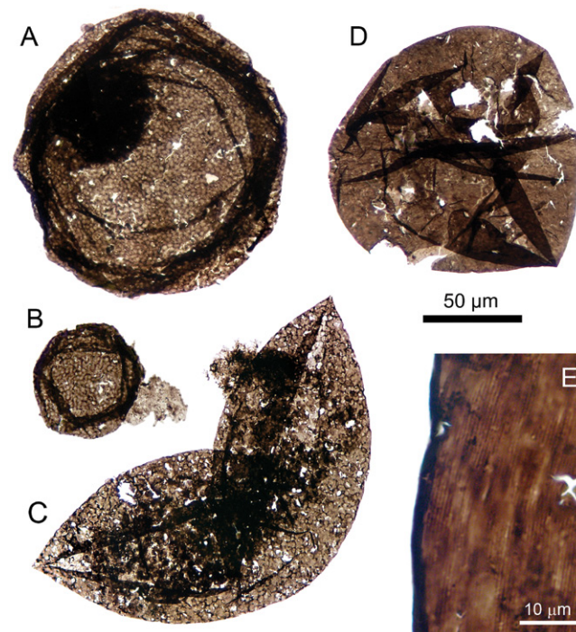
Figure 3. Eukaryotic microfossils from the Greyson Formation (Montana, USA). A–C: Dictyosphaera macroreticulata , with reticulate wall structure, intracellular inclusion (A) and medial split (C). D, E: Valeria lophostriata , with concentric wall microstructure. Dark scale bar applies to A–D.
