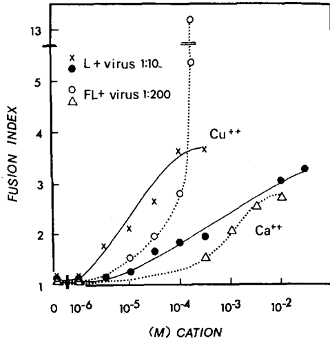
FIGURE 5 Comparison of effects of \text{Cu}^{2+} and \text{Ca}^{2+} on fusion of L and FL cells.
