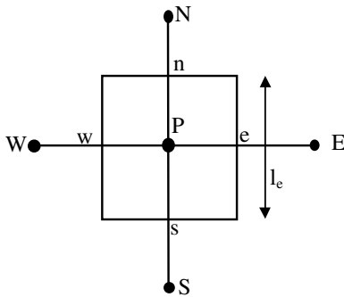
Figure 10 | A control volume around node P.
