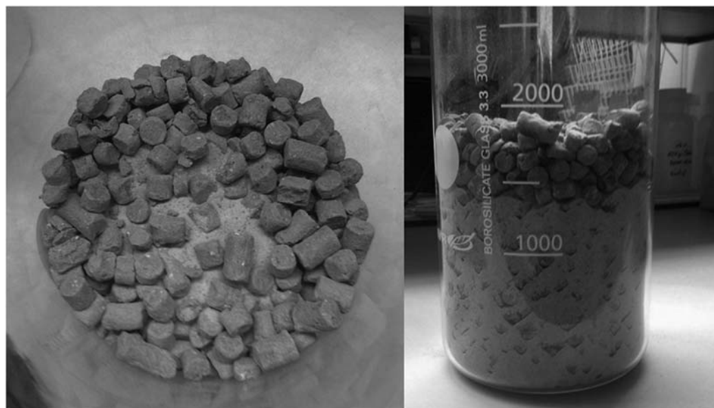
FIG. 9. Emplacement of the bimodal blend in a flask in the laboratory. The silica sand was added after the pellets, without vibration or compaction.
