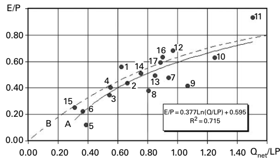
Figure 8 General relationship between the radiation humidity index ( Q_{\text{net}}/LP ) and the ratio of evaporation to precipitation ( E/P ) for northern research basins. Empirical approximation A (see the formula within inset): theoretical equation B (Budyko, 1971): E/P = 1 - \exp(-Q_{\text{net}}/LP) . Study sites: 1 - Valday (Russia), 2 - Brusovitsa (Russia), 3 - Askanjoki (Finland), 4 - Iittovuoma (Finland), 5 - Bayelva (Svalbard, Norway), 6 - Moshiri (Japan), 7 - Mogot (Siberia, Russia), 8 - Kolyma (Siberia, Russia), 9 - Tiksi (Russia), 10 - Dead Creek (Manitoba, Canada), 11 - Wolf Creek (Yukon, Canada), 12 - Ft. Simpson (NWT, Canada), 13 - Caribou Poker Creeks (Alaska, USA), 14 - Imnavait Creek (Alaska, USA), 15 - Baffin Island (Canada), 16 - Devon Island (Canada), 17 - Ellesmere Island (Canada)
