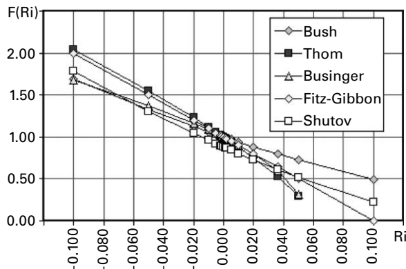
Figure 1 Stability functions F(Ri) offered by several researchers. The most frequent values (more than 90% of all observations) of Ri numbers at Valday range from -0.020 to 0.080
