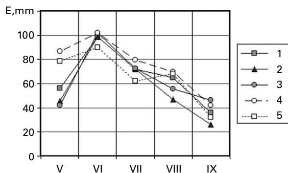
Figure 4 Monthly evaporation rates for a summer season at Valday. 1 - water surface evaporation as measured with the use of 20\text{ m}^2 area basin, 2 - grassland evapotranspiration measured directly by weighing lysimeters, 3 - grassland evapotranspiration determined by the energy balance method, 4, 5 - evapotranspiration calculated by Budyko (1971) and Shutov (1998) respectively
