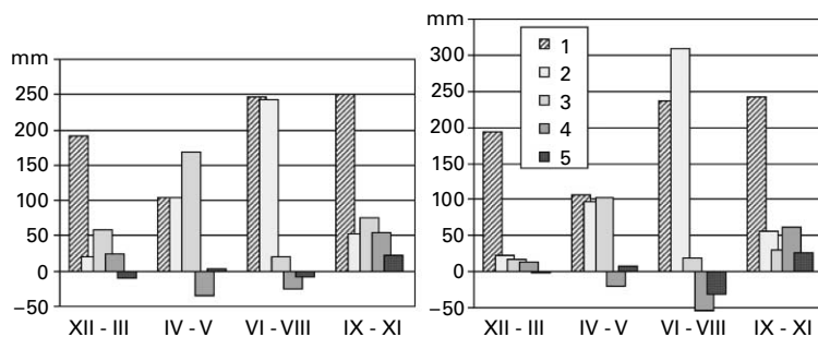
Figure 6 Seasonal water balance components at Valday, Russia, observed for grassland (on the left) and forested watersheds (on right, Balonishnikova et al. 2004). 1 - precipitation ( P ), 2 - evapotranspiration ( ET ), 3 - runoff ( Q ), 4 - soil moisture change ( \Delta SM ), 5 - ground water storage change ( \Delta GW )
