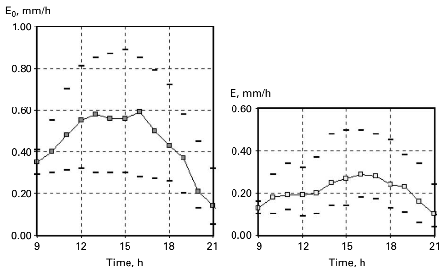
Figure 2 Time-averaged daily courses of potential ( E_0 , on the left) and actual evaporation ( E , on the right) by the ASDSA measurements. Dashes show possible deviations from average
