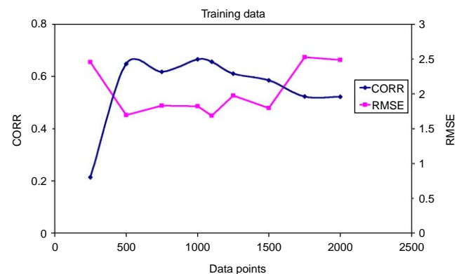
Figure 7 | Variation of CORR and RMSE in data splitting analysis in validation data range.
