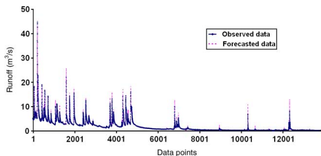
Figure 9 | Observed and 4-h-ahead forecasted runoff of the study area using data with 30 min sampling frequency.
