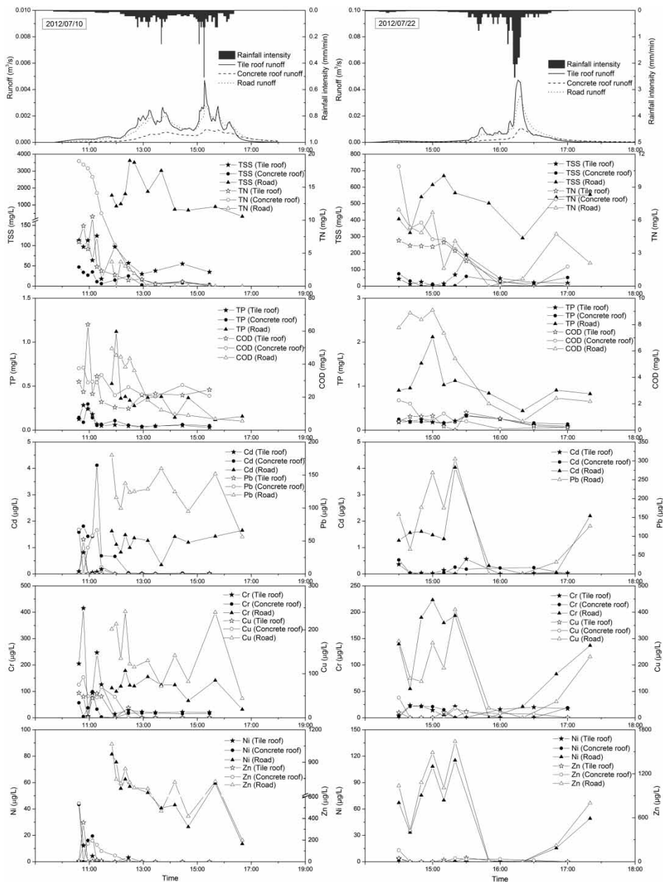
Figure 2 | Hydrographs and pollutographs for the different surfaces for the July 10 and July 22 events.
