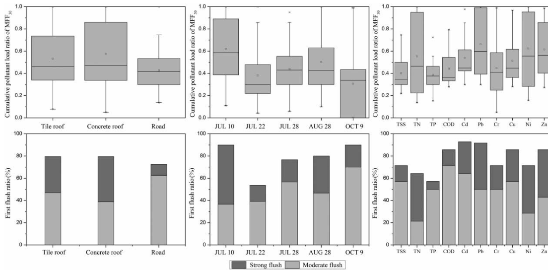
Figure 4 | The MFF_{30} cumulative pollutant load and FF probability of different sampling sites, rainfall events and pollutants. Moderate flush: 1 < MFF_{30} < 2 ; strong flush: MFF_{30} \geq 2 . FF ratio refers to the moderate and strong flush events as a proportion of the total event.
