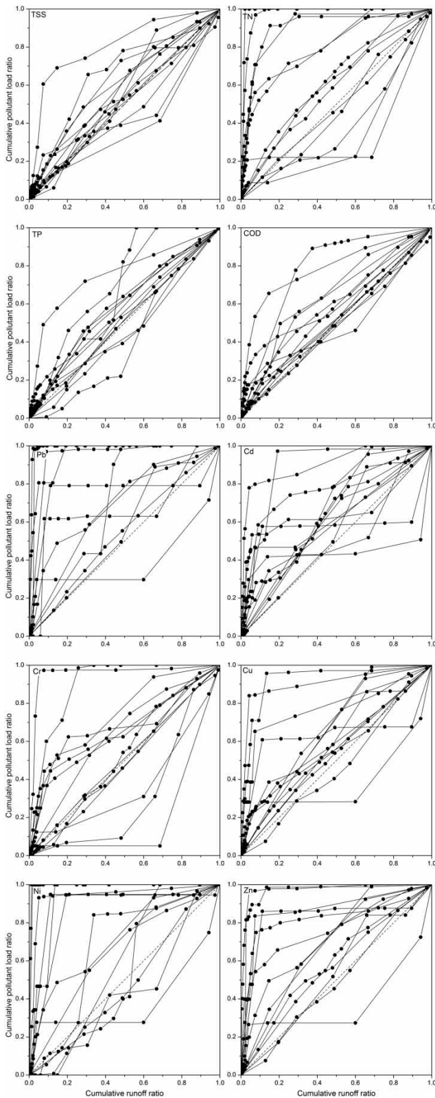
Figure 3 | M(V) curves for pollutants in different runoffs.
