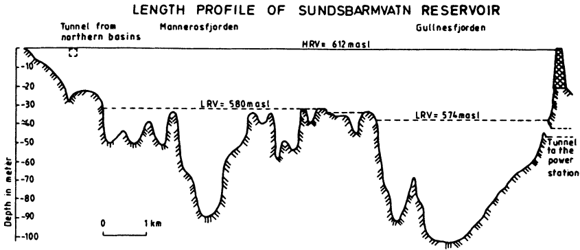
Fig. 2. Length profile of Sundsbarmvatn Reservoir along the deepest parts. The water level at the highest and lowest regulated water level (HRV and LRV) are marked.
