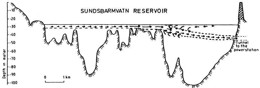
Fig. 6. The flow pattern in Sundsbarmvatn Reservoir at the end of the winter period as interpreted from the temperature measurements
