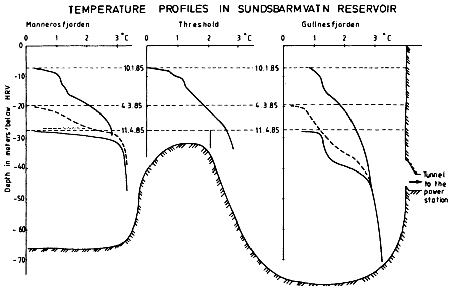
Fig. 3. The water level and the temperature profiles as measured on 10 January, 4 March and 11 April in Mannerosfjorden, at the threshold and in Gullnesfjorden. Compare with Figs. 1 and 2.
