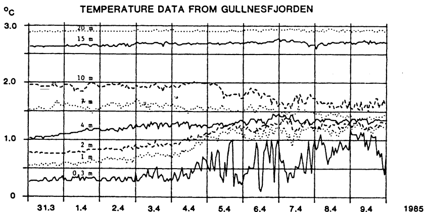
Fig. 5. Temperature curves from the upper 8 of the 11 depths recorded every hour in Gullnesfjorden. The curves show the temperature pattern at the end of the winter period. The depths are in metres below the ice.
