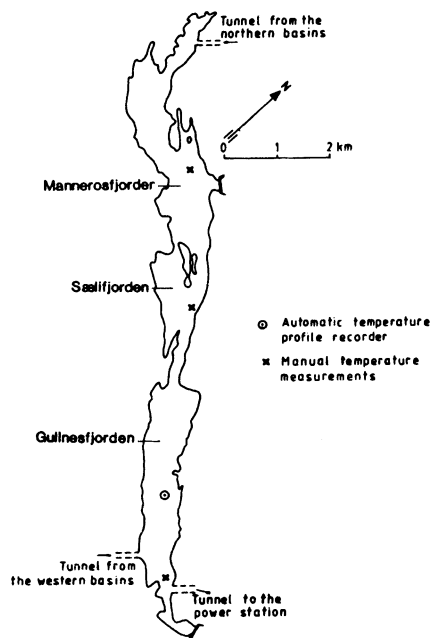
Fig. 1. Map showing the Sundsbarmvatn Reservoir at maximum water level. The position of the temperature measurements referred to in the text is marked.
