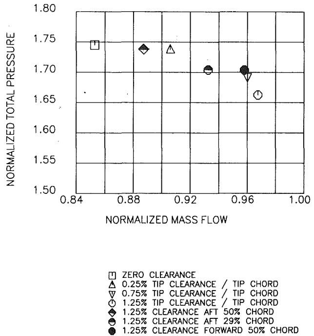
Fig. 19 Predicted pressure ratio at near-stall points for tip clearance/tip chord ratios of zero, 0.25 percent, 0.75 percent, and clearance of 1.25 percent aft of 29 percent and 50 percent chord and forward of 50 chord
