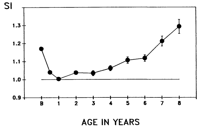
FIG. 3. Symmetry index (SI) (mean \pm SEM) in offspring of diabetic mothers from birth to 8 yr of age. SI is greater than expected (1.0) at all ages except 12 mo ( P < 0.05 ). Data points are means \pm SE.
