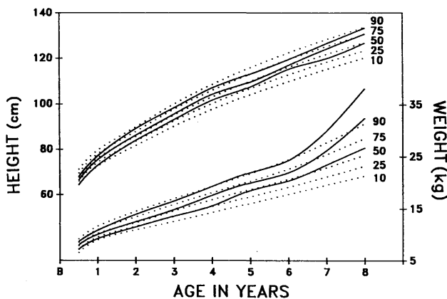
FIG. 2. Physical growth of male offspring of diabetic mothers (ODM). Dotted lines, National Center for Health Statistics 90th, 75th, 50th, 25th, and 10th percentiles for American boys; solid lines, 75th, 50th, and 25th percentiles for male ODM for height (upper curves) and weight (lower curves).
